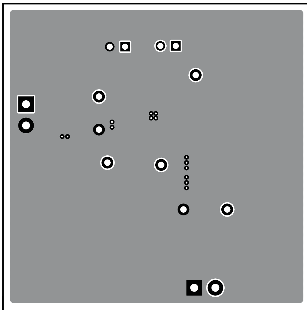
Figure 13. TPS54418EVM-375 Layout 2
