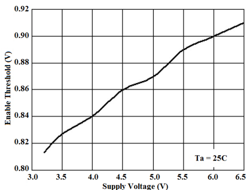
Fig. 12: Enable Threshold vs. Supply Voltage
