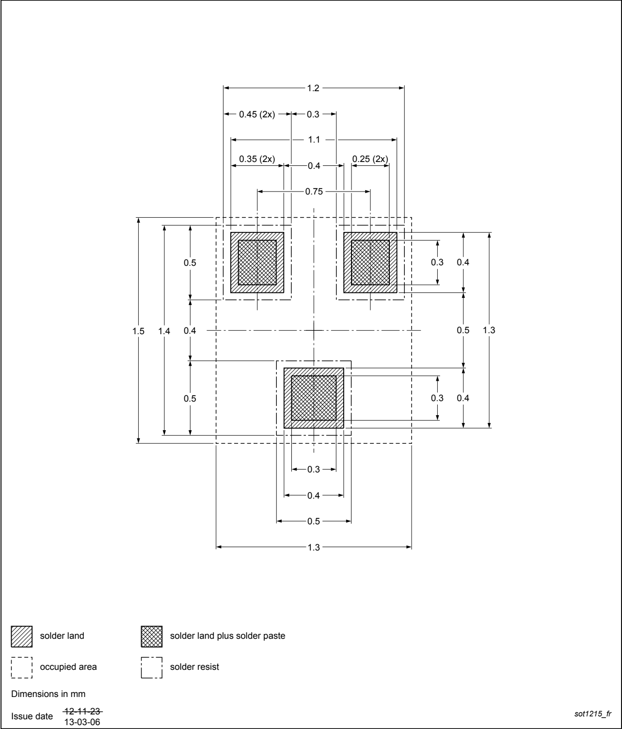
Fig. 13. Reflow soldering footprint for DFN1010D-3 (SOT1215)
