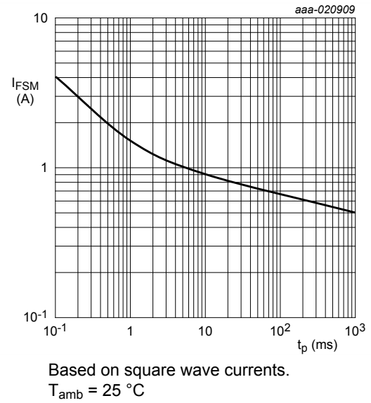
Fig. 5. Non-repetitive forward current as a function of pulse duration; maximum values
