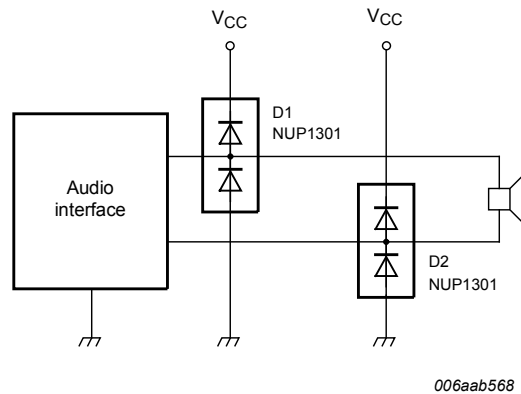
Fig. 11. Typical application for the protection of one signal line
