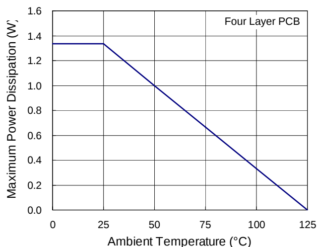
Figure 3. Derating Curves for RT8265 Packages
