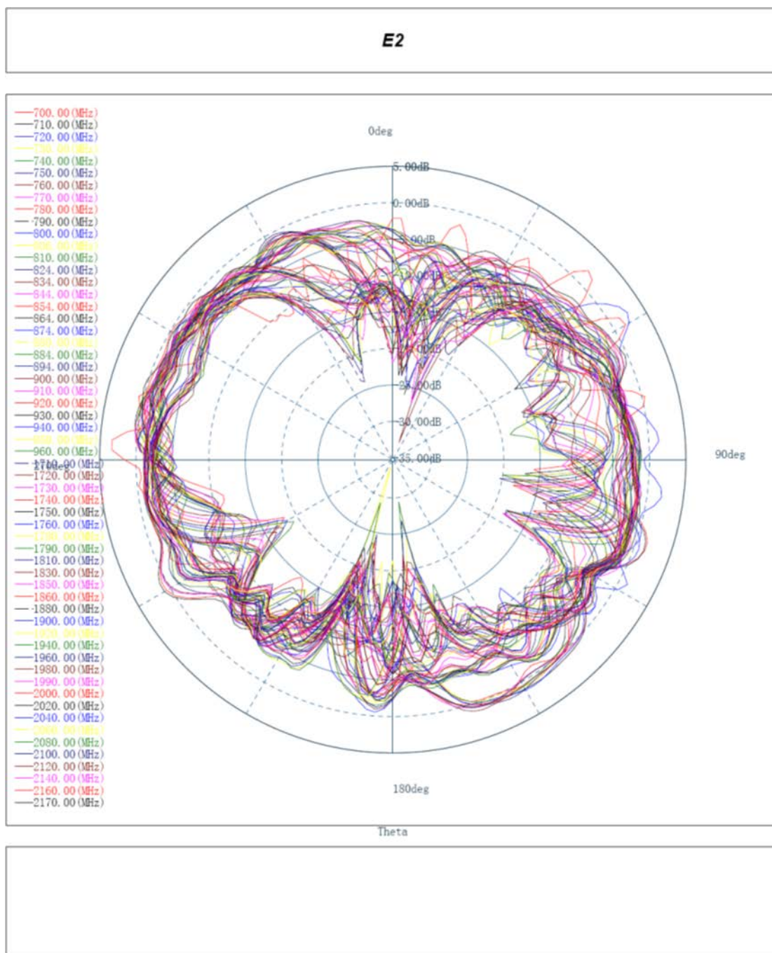
Figure 26 Radiation Pattern E-plane (E2)
