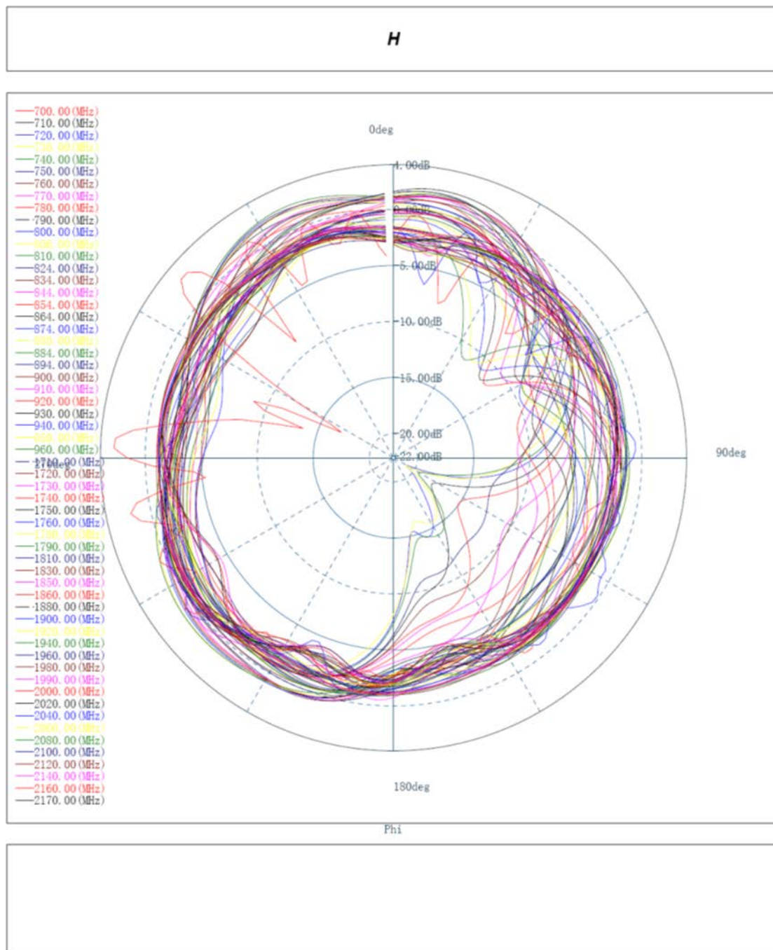
Figure 24 Radiation Pattern H-plane
