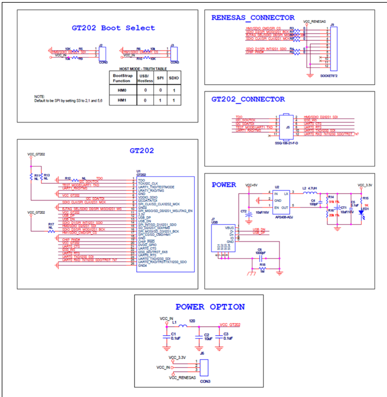
Figure 18 Wi-Fi Board Schematic
