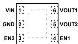
ISL9016 (6 LD 1.6x1.6 \mu TDFN) TOP VIEW
