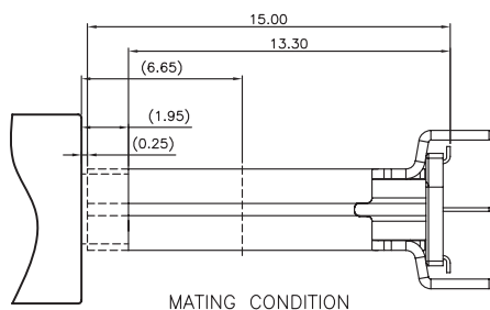
MATING CONDITION
