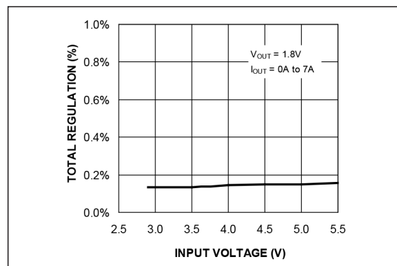
FIGURE 2-4: Load Regulation vs. Input Voltage.
