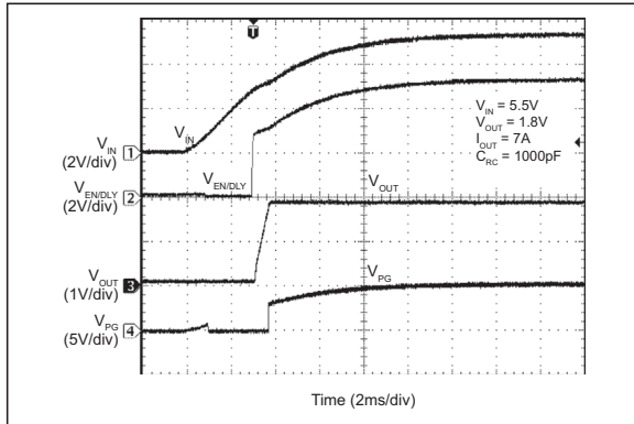
FIGURE 2-31: V IN Turn-On.
