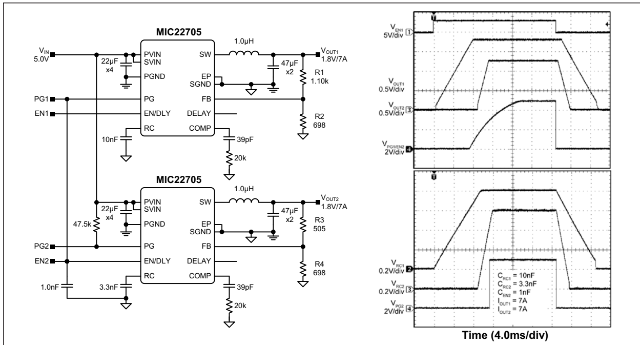
FIGURE 4-7: Delayed Sequencing.
