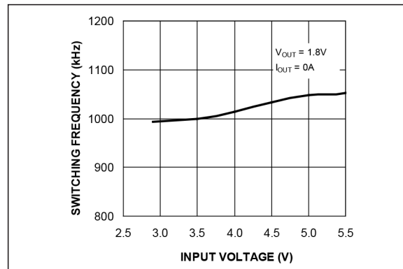
FIGURE 2-6: Switching Frequency vs. Input Voltage.
