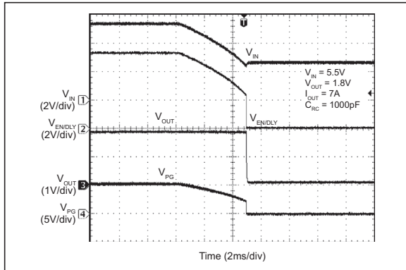
FIGURE 2-32: V IN Turn-Off.
