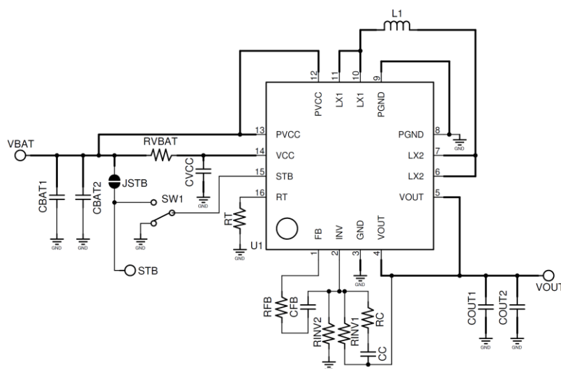
Figure 2. BD8306MUV-EVK-001 Schematic
