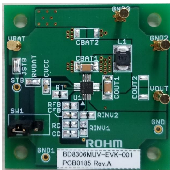
Figure 1. BD8306MUV-EVK-001
