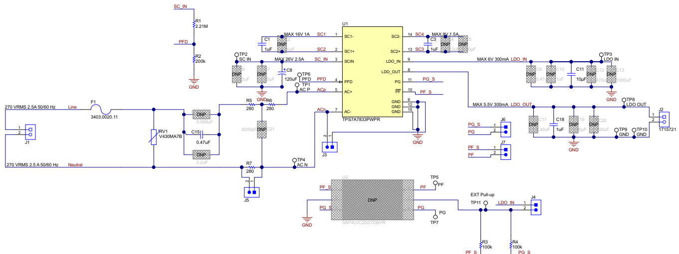
Figure 1. TPS7A78EVM-011 Schematic
