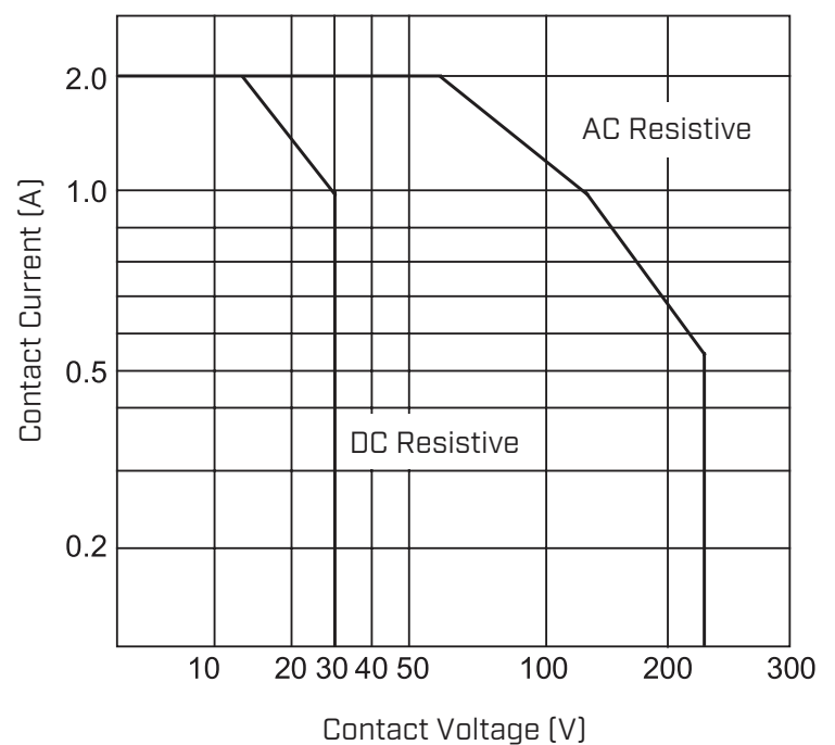
Maximum Switching Power
