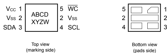
Figure 2. 5-pin package connection
