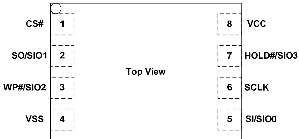
Figure 1-4. Pin Assignments
