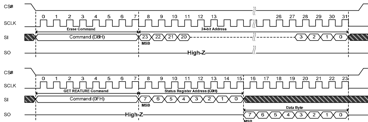
Figure 9-1. Block Erase (D8H) Sequence Diagram
