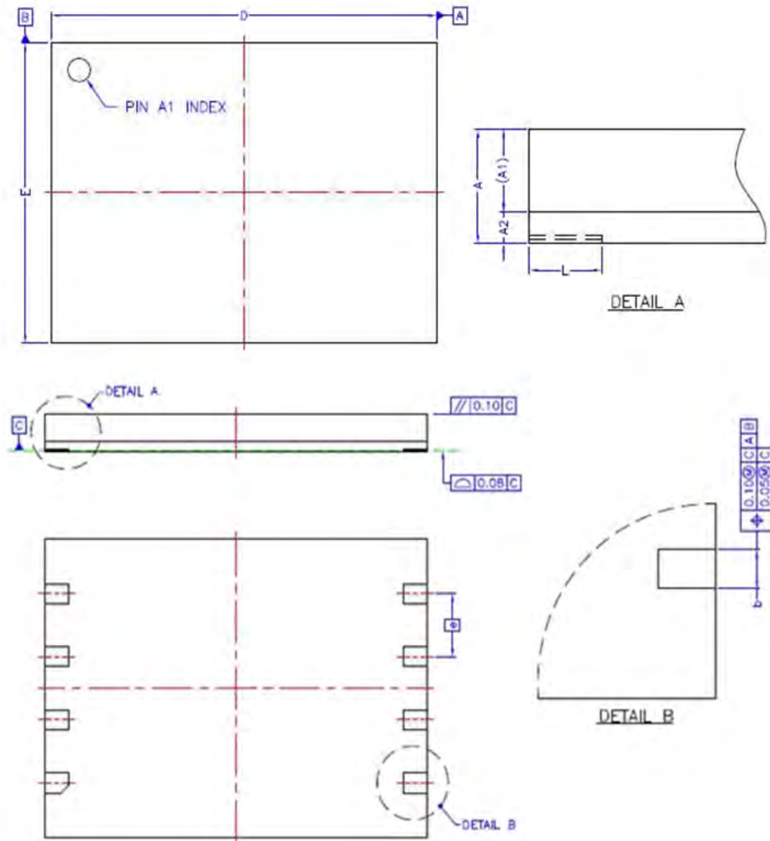
Figure 17-1. LGA (8x6x0.8mm) Package Outline Drawing Information
