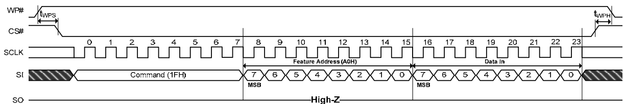
Figure 16-4. WP# Timing
