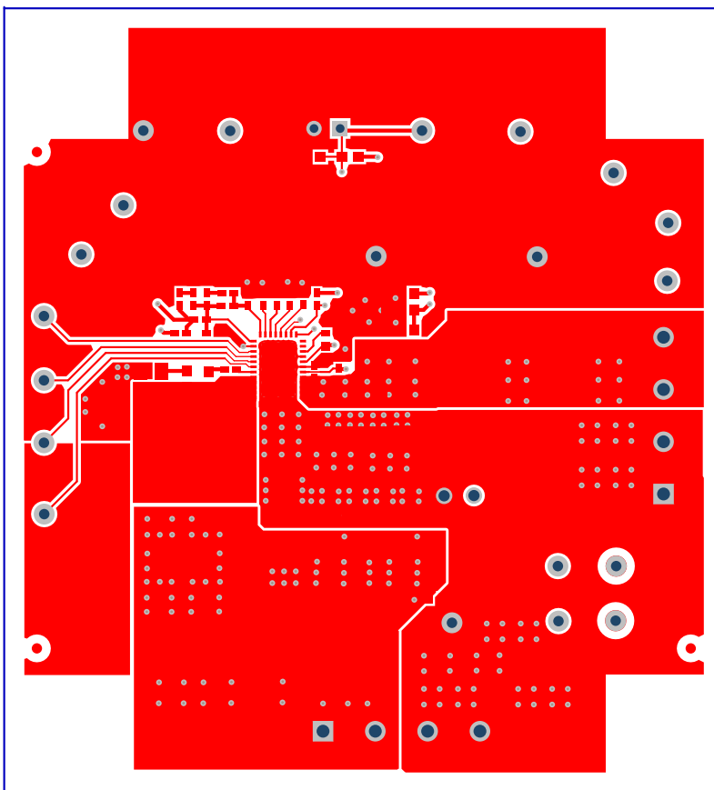
Figure 10-3. BSR054EVM Top Layer (Top View)
