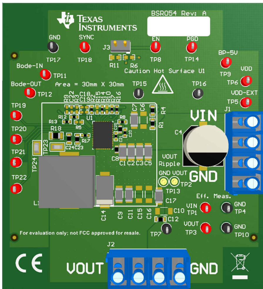
Figure 6-1. BSR054EVM Overview
