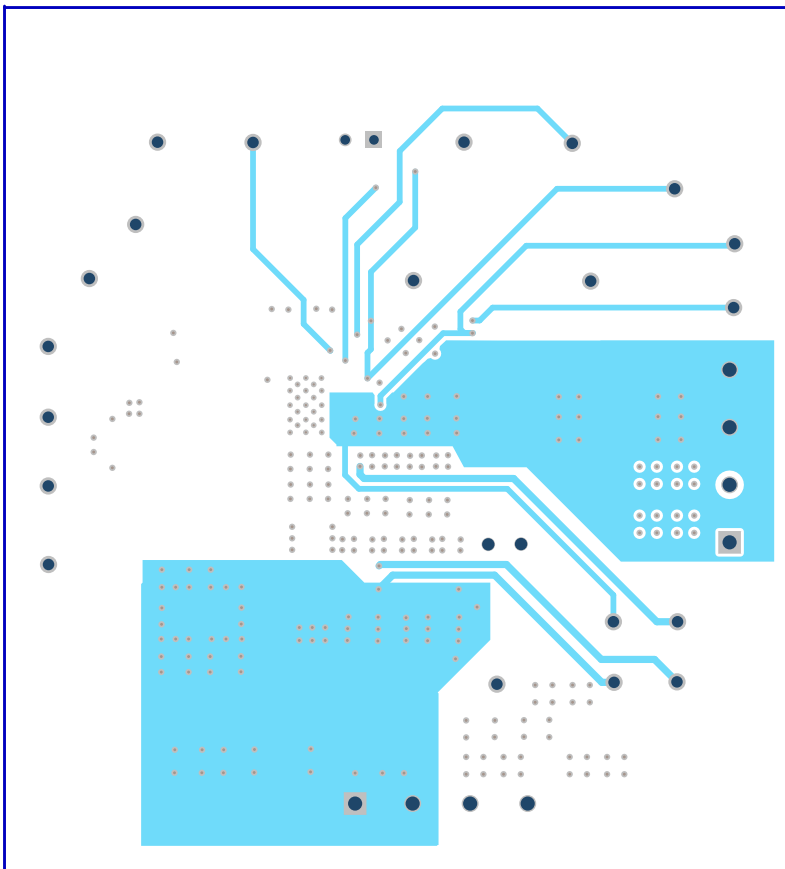
Figure 10-5. BSR054EVM Inner Layer 2 (Top View)
