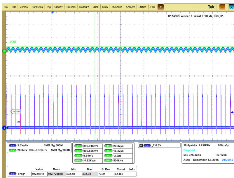
Figure 9-6. Output Ripple and SW Node of 0.9-V Output at 12-V IN , 0-A Output
