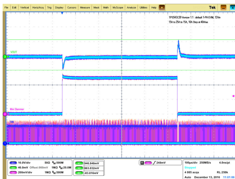
Figure 9-4. Transient Response of 0.9-V Output at 12-V IN , Transient is 15 A to 25 A to 15 A, the Step is 10 A at 40 A/μs
