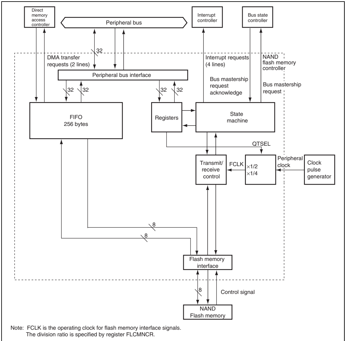
Figure 26.1 Block Diagram
