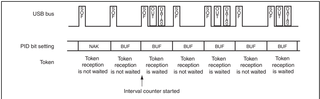
Figure 27.19 Relationship between (μ) Frames and Expected Token Reception when IITV = 1
