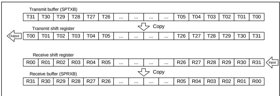
Figure 17.8 LSB First Transfer (32-Bit Data)
