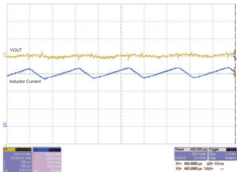
Figure 2. Output Voltage Ripple, V_{in}=3 V, V_{out}=1.8 V, I_{load}=600 mA
