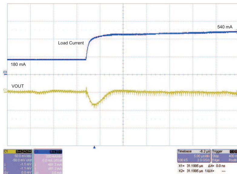
Figure 4. Load Transient, 180-mA to 540-mA Step
