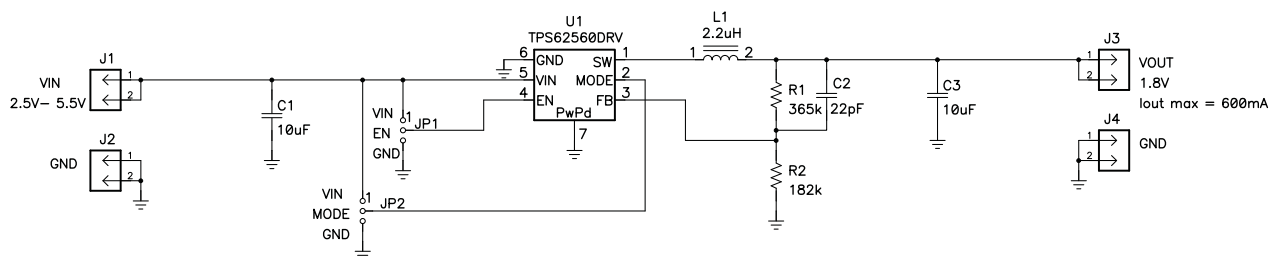
Figure 8. TPS62560EVM-330 Schematic
