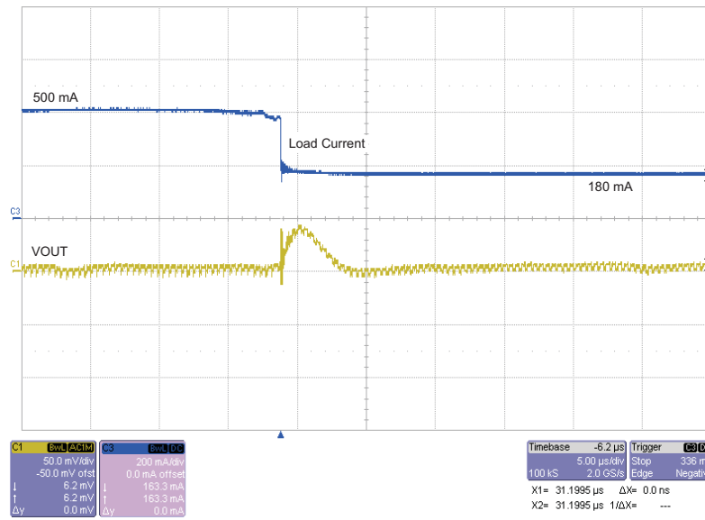
Figure 3. Load Transient, 500-mA to 180-mA Step, V_{in}=3 V, V_{out}=1.8 V
