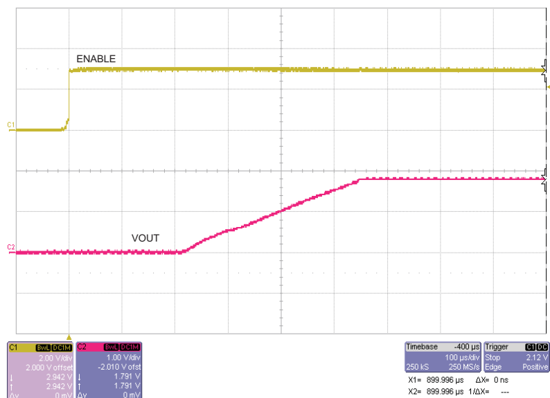
Figure 1. Start-up From Enable, V_{in}=3 V, V_{out}=1.8 V, I_{load}=600 mA
