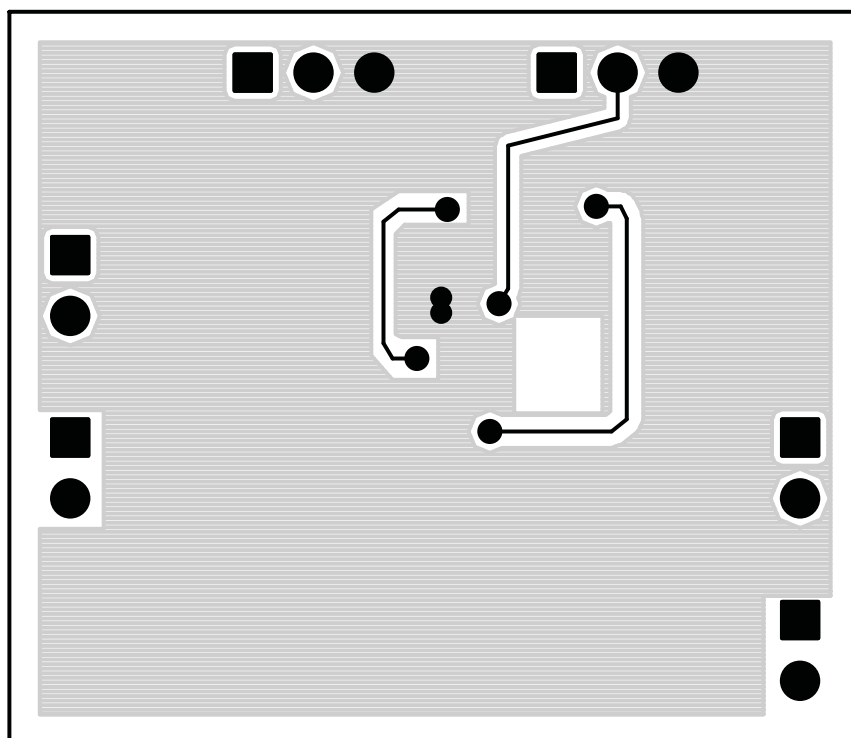
Figure 7. Bottom Layer Routing
