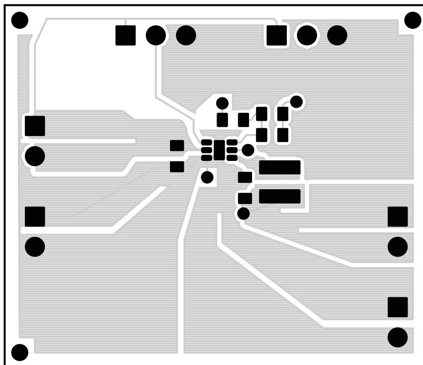
Figure 6. Top Layer Routing
