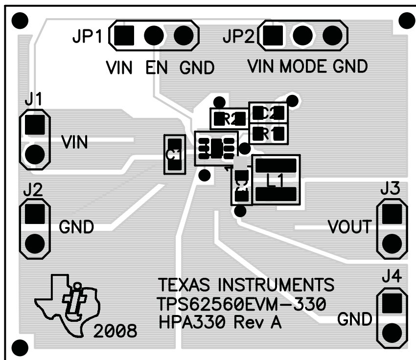
Figure 5. Assembly Layer
