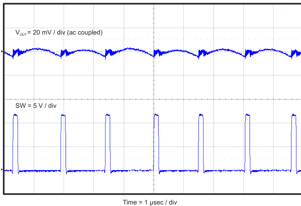
Figure 4-7. TPS56528EVM-534 Output Voltage Ripple ( I_{OUT} = 500 \text{ mA} )
