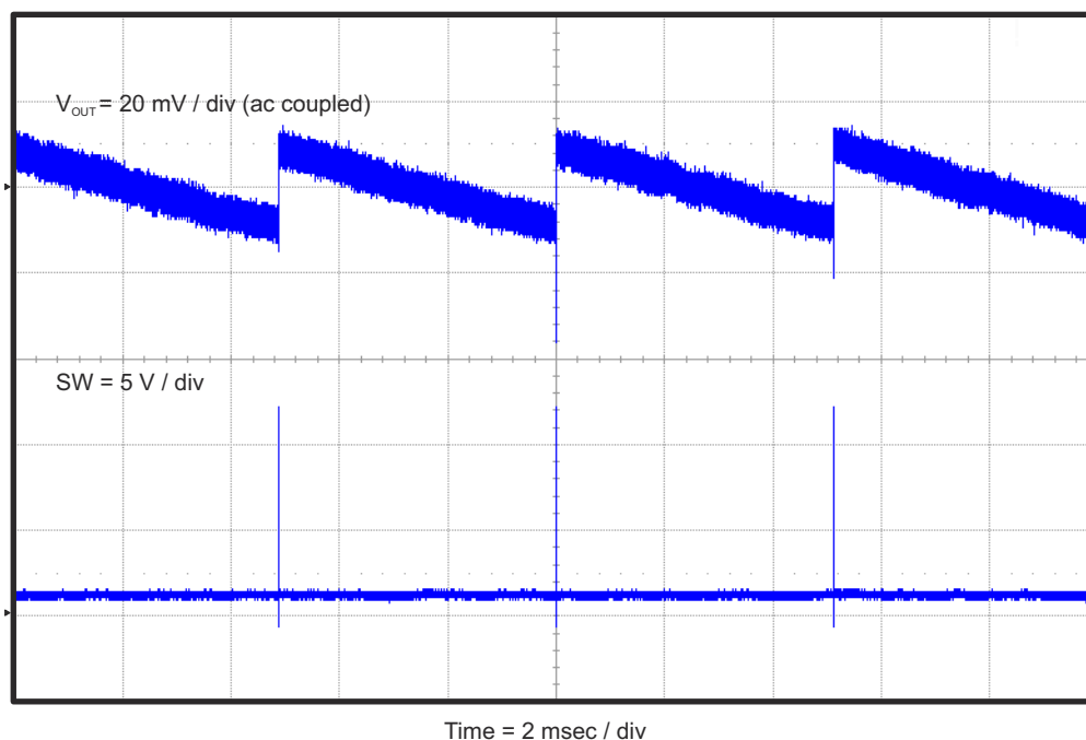
Figure 4-8. TPS56528EVM-534 Output Voltage Ripple ( I_{OUT} = 1 mA)
