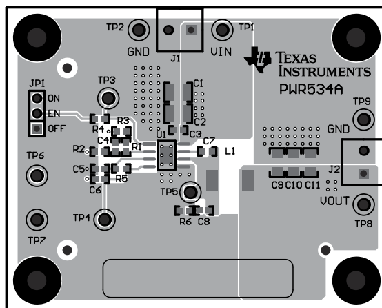
Figure 5-1. Top Assembly
