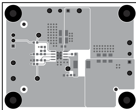
Figure 5-2. Top Layer
