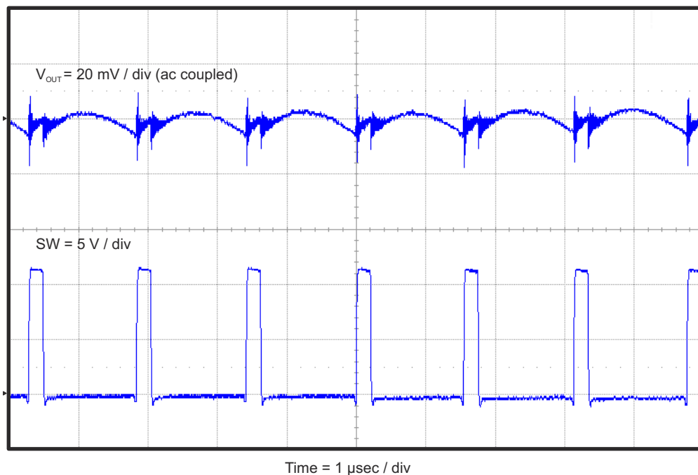
Figure 4-6. TPS56528EVM-534 Output Voltage Ripple ( I_{OUT} = 5 \text{ A} )
