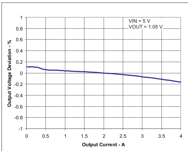
Figure 4-3. TPS54425EVM-608 Load Regulation
