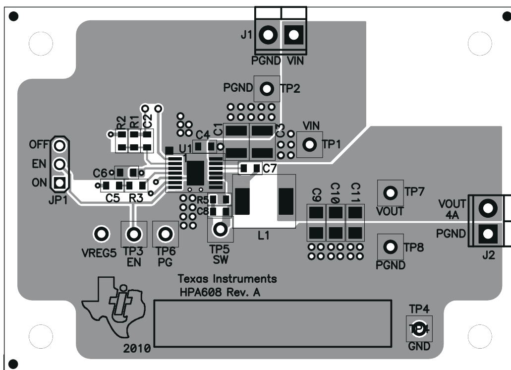
Figure 5-1. Top Assembly
