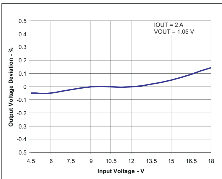
Figure 4-4. TPS54425EVM-608 Line Regulation
