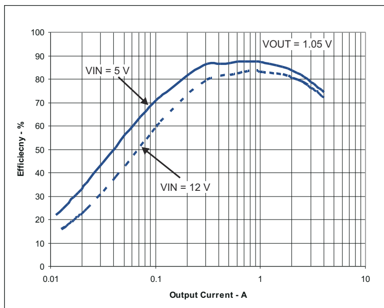
Figure 4-2. TPS54425EVM-608 Light Load Efficiency
