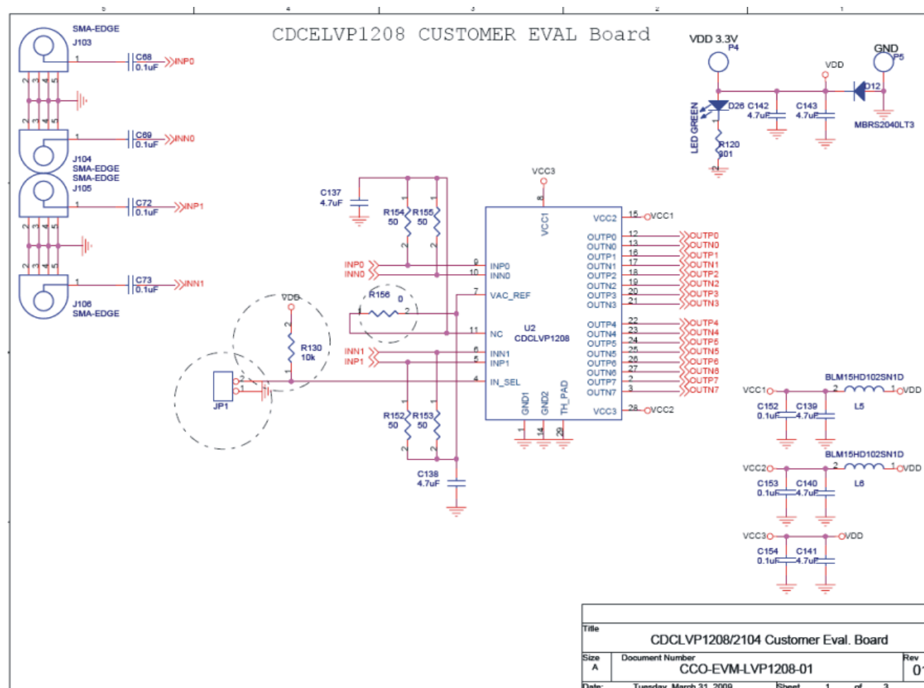
Figure 2. CDCLVP1208EVM—Schematic
