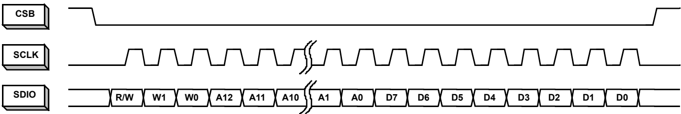
FIGURE 39. MSB-FIRST ADDRESSING
