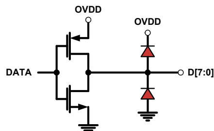
FIGURE 52. CMOS OUTPUTS
