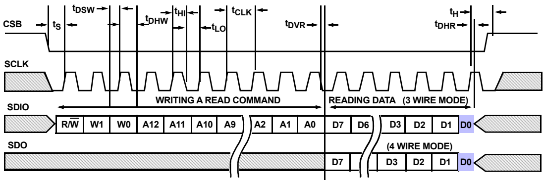
SPI READ
