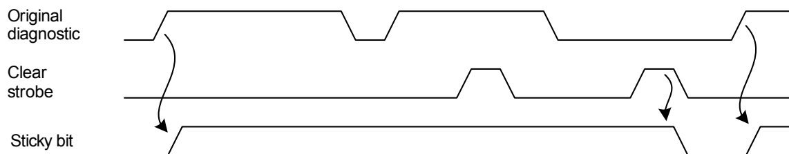
Registers - sticky_bit_def
