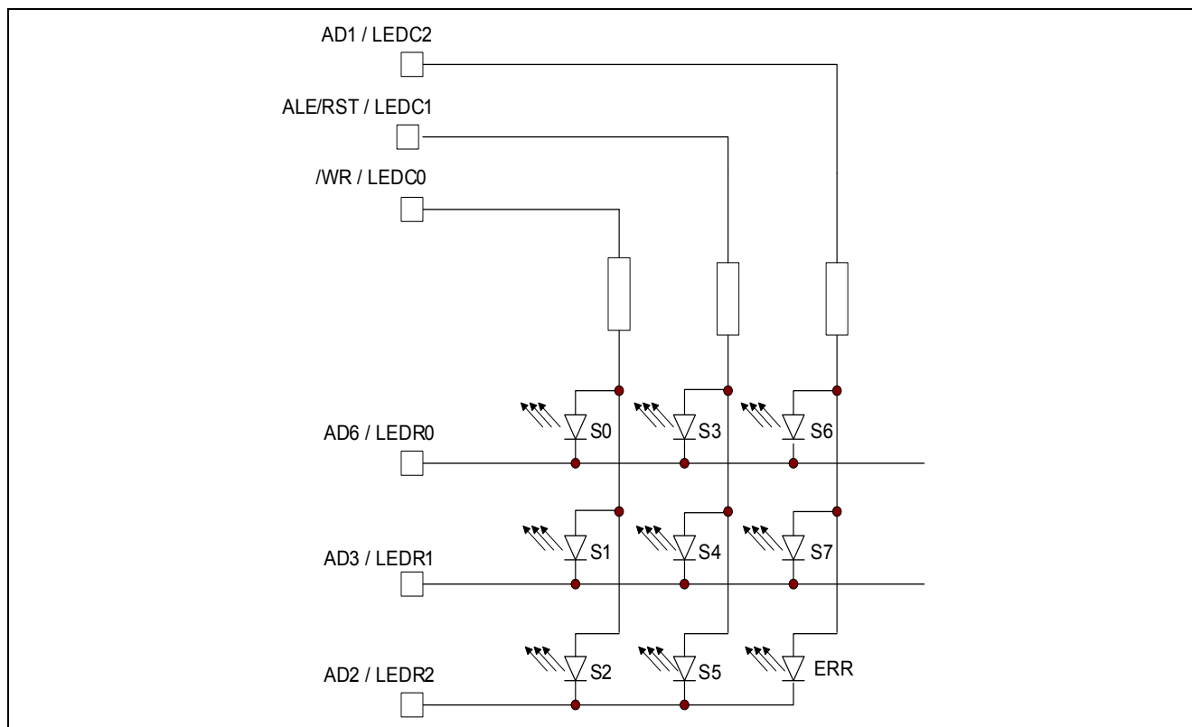
Figure 25 LED Matrix connected to the uC-Chip
