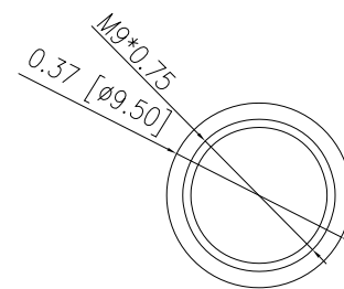
BACK SHELL
