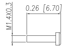
SCREW
