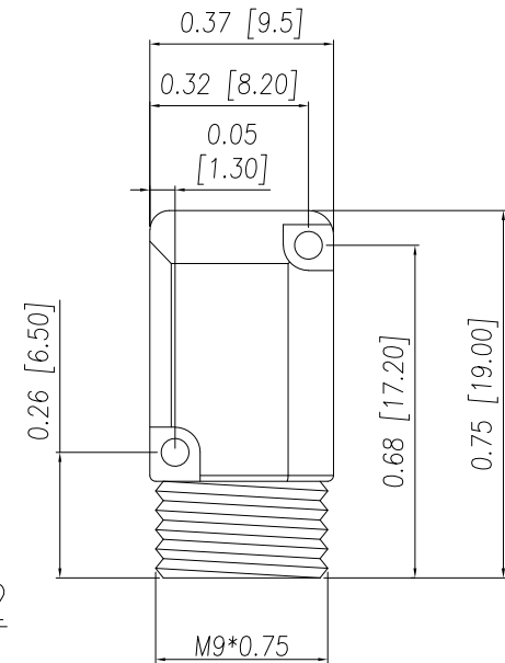
COVER 2
