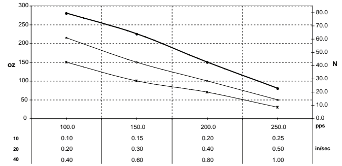
42DBLXXCXB-K/L Typical pull-in linear force vs linear rate at 20°C Full step, Bipolar, L/R drive
