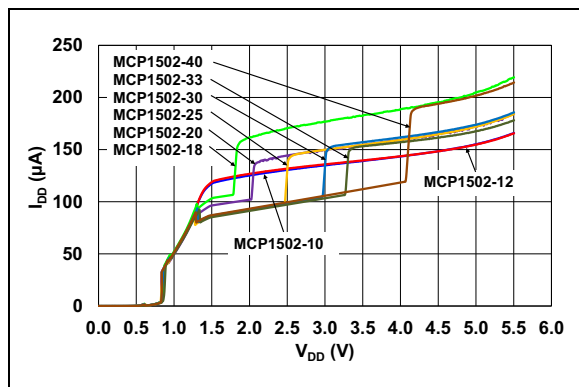
FIGURE 3-7: I_{DD} vs. V_{DD} for All Options.
