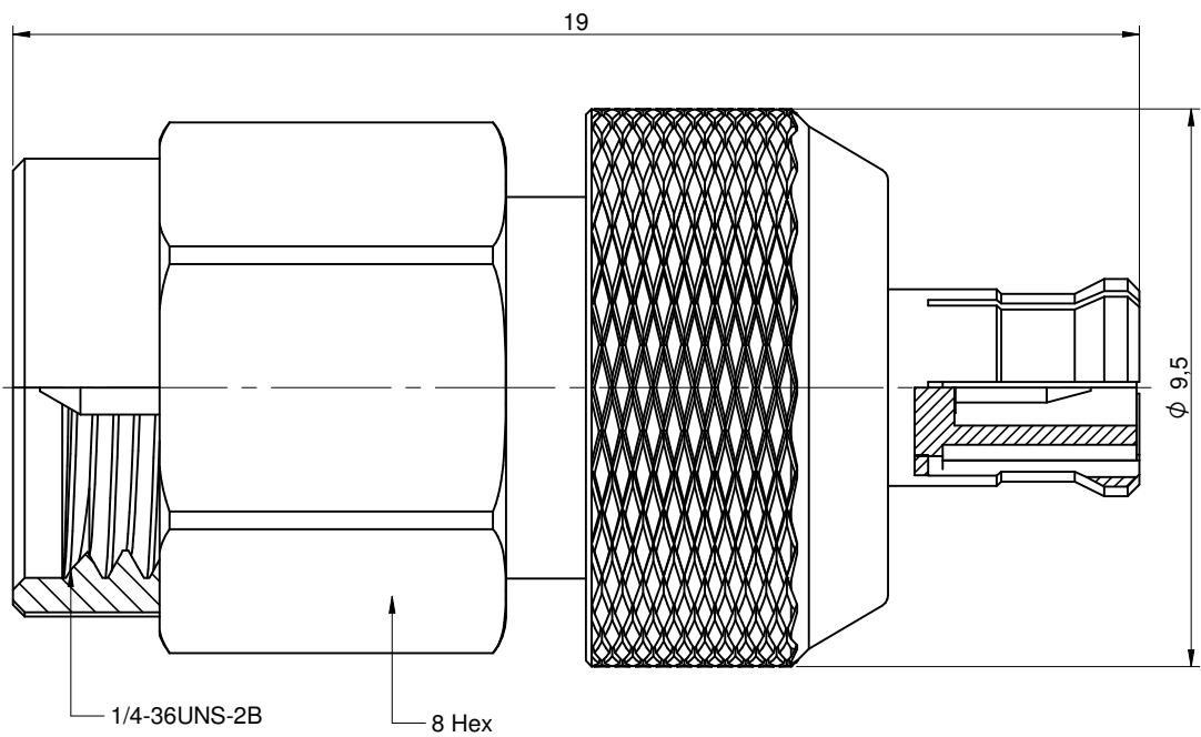
Connector 1
