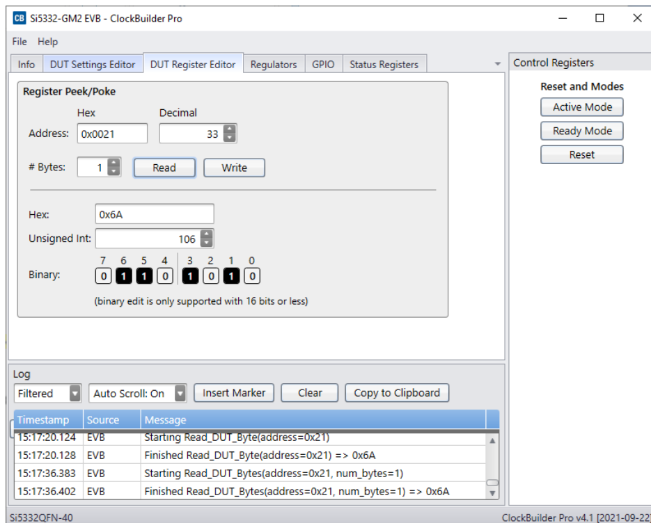
Figure 4.2. Register Access
