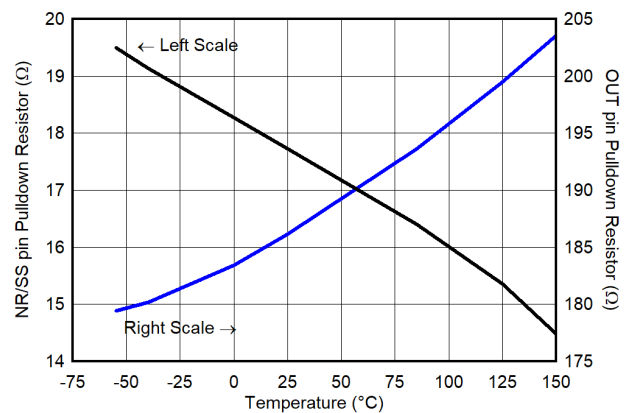
Figure 6-104. NR/SS and OUT Pulldown Resistors vs Temperature
