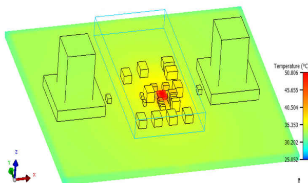
Figure 8-25. TPS7A94EVM-046 Device Thermal Gradient
