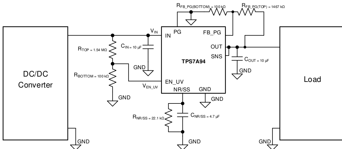
Figure 8-26. Typical Application Circuit
