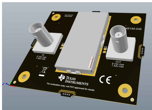
Figure 8-23. TPS7A94EVM-046 3D View
