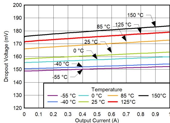
Figure 6-42. Dropout Voltage vs I_{OUT} for V_{OUT} = 1.8 V
