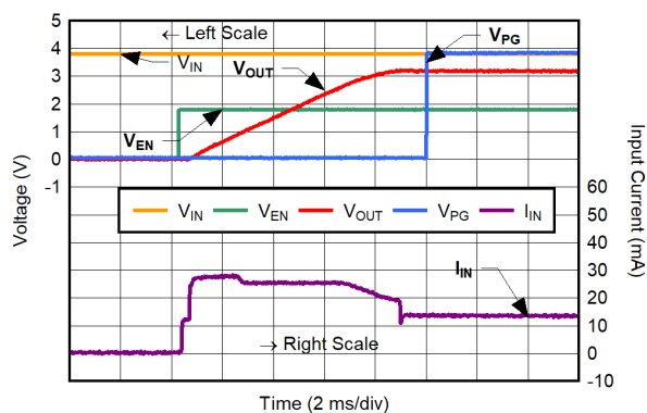
Figure 6-37. Inrush Current for C_{NR/SS} = 1.0 \mu F
