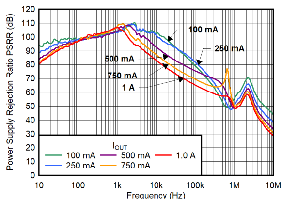
Figure 8-13. PSRR vs Frequency and I_{OUT} for V_{OUT} = 3.3 V, C_{OUT} = 10 \mu F
