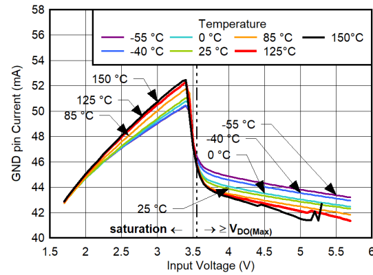
Figure 6-78. GND Pin Current vs V_{IN} and Temperature for I_{OUT} = 1\text{ A}
