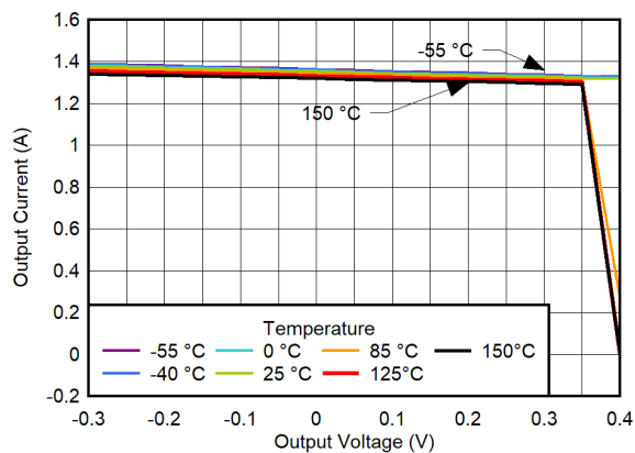
Figure 6-81. 100% Current Limit vs Temperature for V_{OUT} = 0.4\text{ V}
