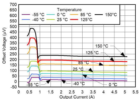
Figure 6-52. V_{OS} vs I_{OUT} and Temperature for V_{NR/SS}
