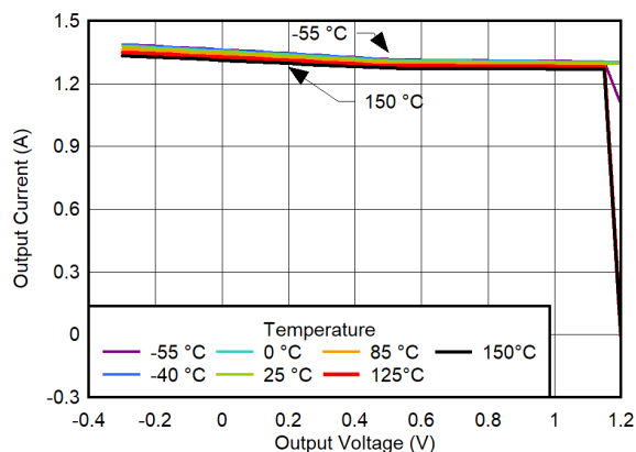
Figure 6-83. 100% Current Limit vs Temperature for V_{OUT} = 1.2\text{ V}
