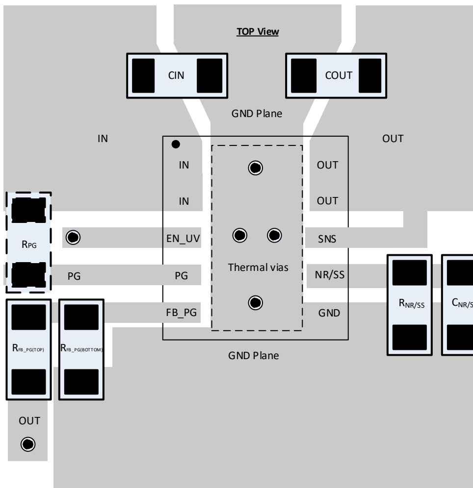
Figure 10-1. Example Layout
