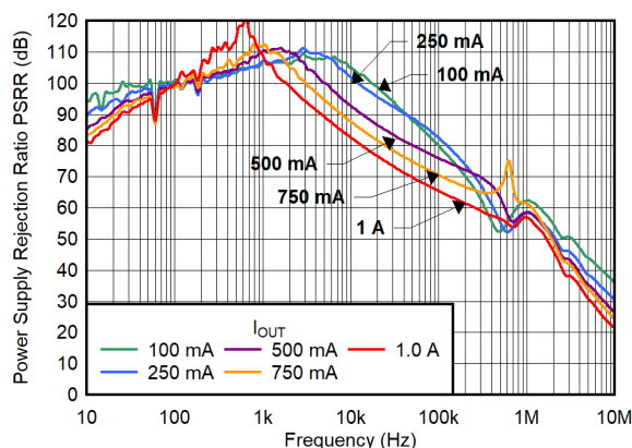
Figure 8-14. PSRR vs Frequency and I_{OUT} for V_{OUT} = 3.3 V, C_{OUT} = 4.7 \mu F || 4.7 \mu F || 1.0 \mu F
