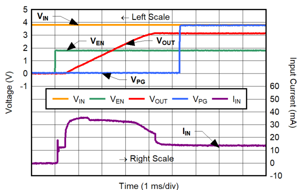
Figure 6-38. Inrush Current for C_{NR/SS} = 2.2 \mu F
