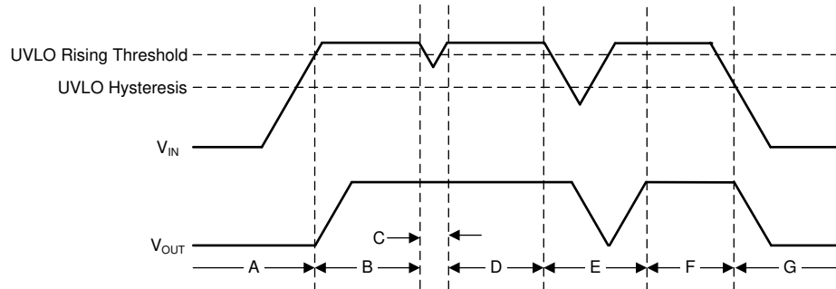
Figure 8-7. Typical UVLO Operation
