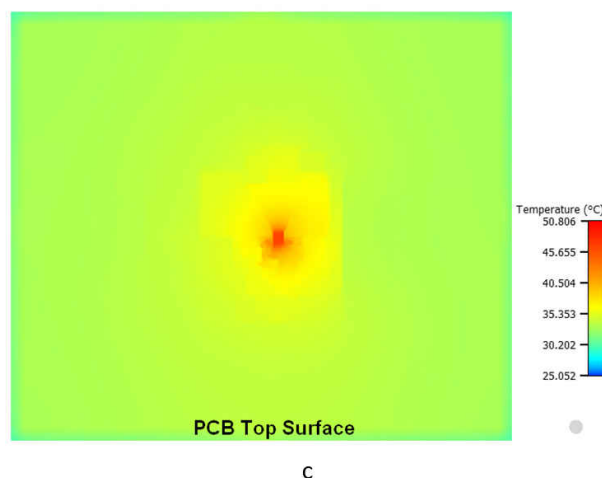
Figure 8-24. TPS7A94EVM-046 PCB Thermal Gradient
