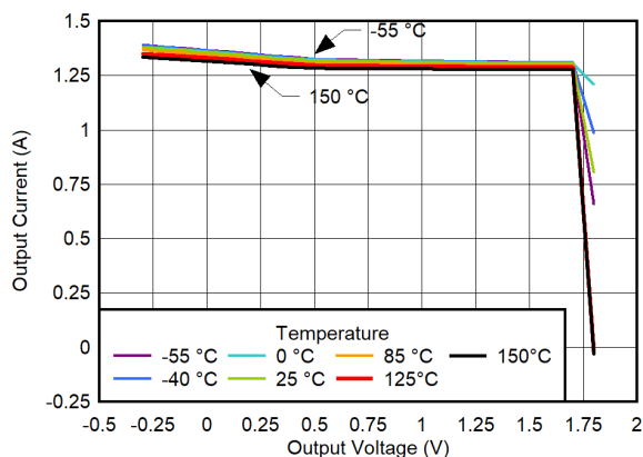
Figure 6-84. 100% Current Limit vs Temperature for V_{OUT} = 1.8\text{ V}
