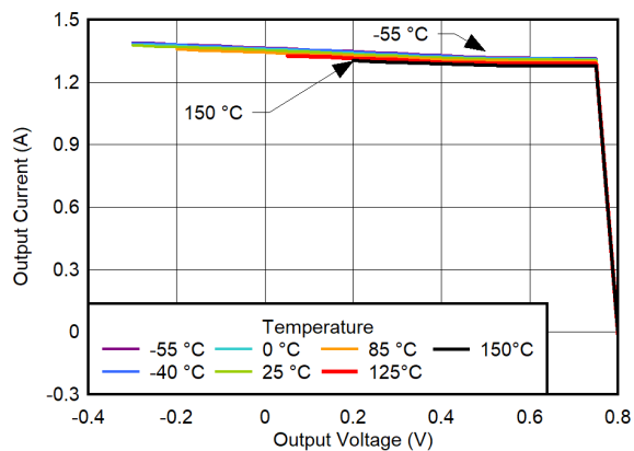
Figure 6-82. 100% Current Limit vs Temperature for V_{OUT} = 0.8\text{ V}
