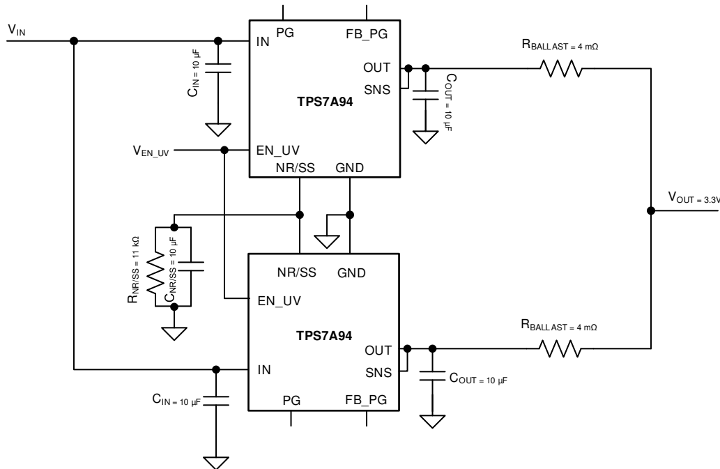
Figure 8-16. Paralleling Multiple TPS7A94 Devices
