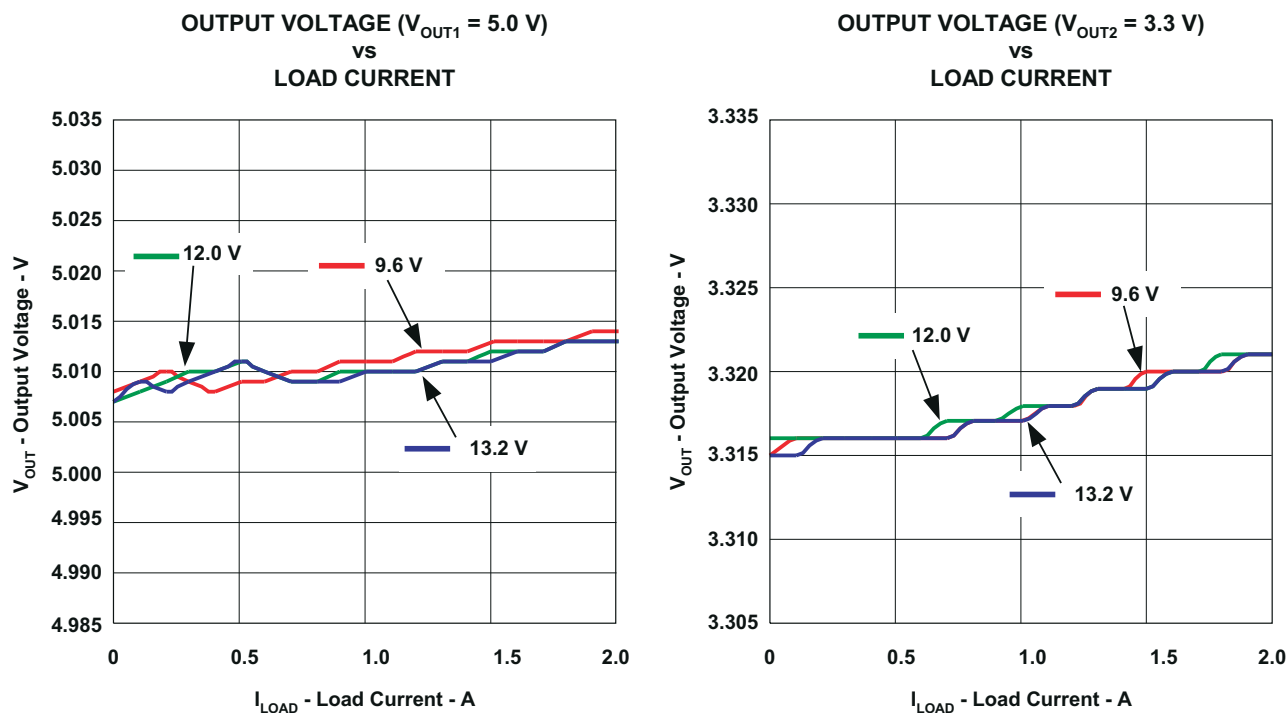
Figure 5-2. TPS54383EVM Output Voltage versus Load Current V_{IN} = 9.6\text{--}13.2 \text{ V} , V_{OUT1} = 5.0 \text{ V} I_{OUT1} = 0\text{--}2 \text{ A} , V_{OUT2} = 3.3 \text{ V} I_{OUT2} = 0\text{--}2 \text{ A}
