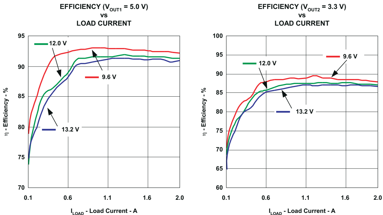
Figure 5-1. TPS54383EVM Efficiency verse Load Current V_{IN} = 9.6\text{-}13.2 \text{ V} , V_{OUT1} = 5.0 \text{ V} I_{OUT1} = 0\text{-}2 \text{ A} , V_{OUT2} = 3.3 \text{ V} I_{OUT2} = 0\text{-}2 \text{ A}
