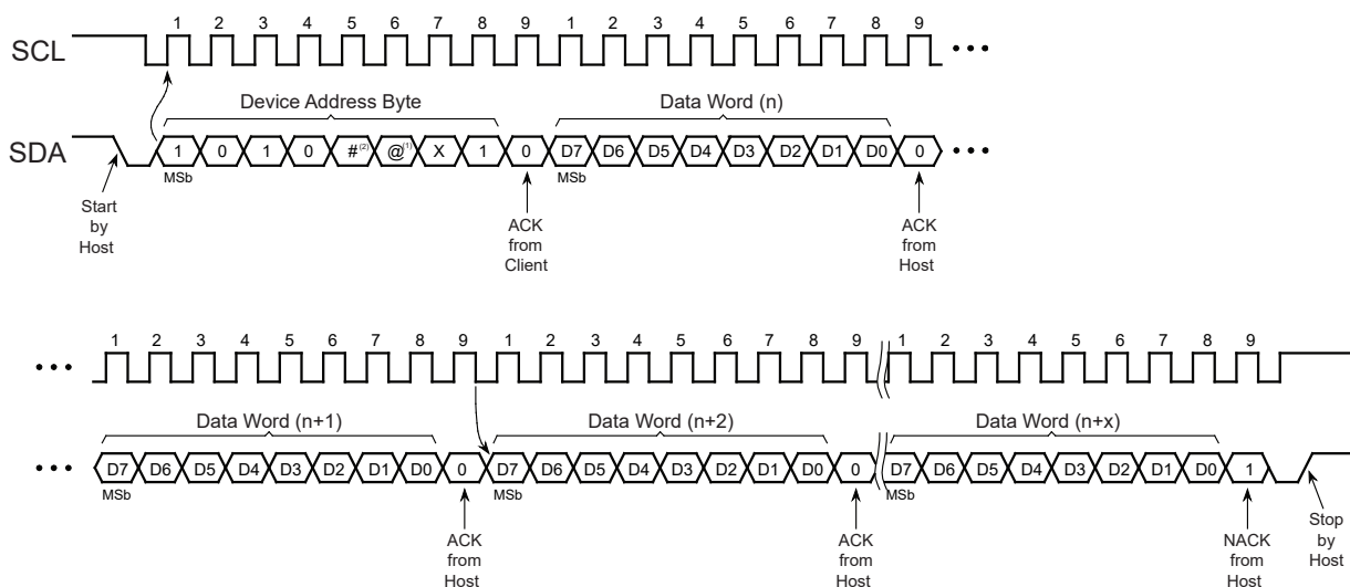
Figure 9-3. Sequential Read
