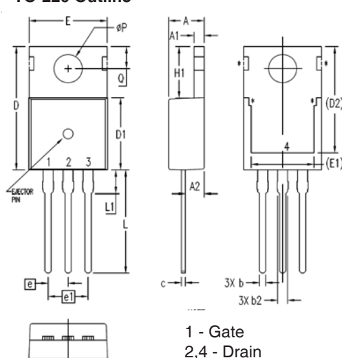
TO-220 Outline
