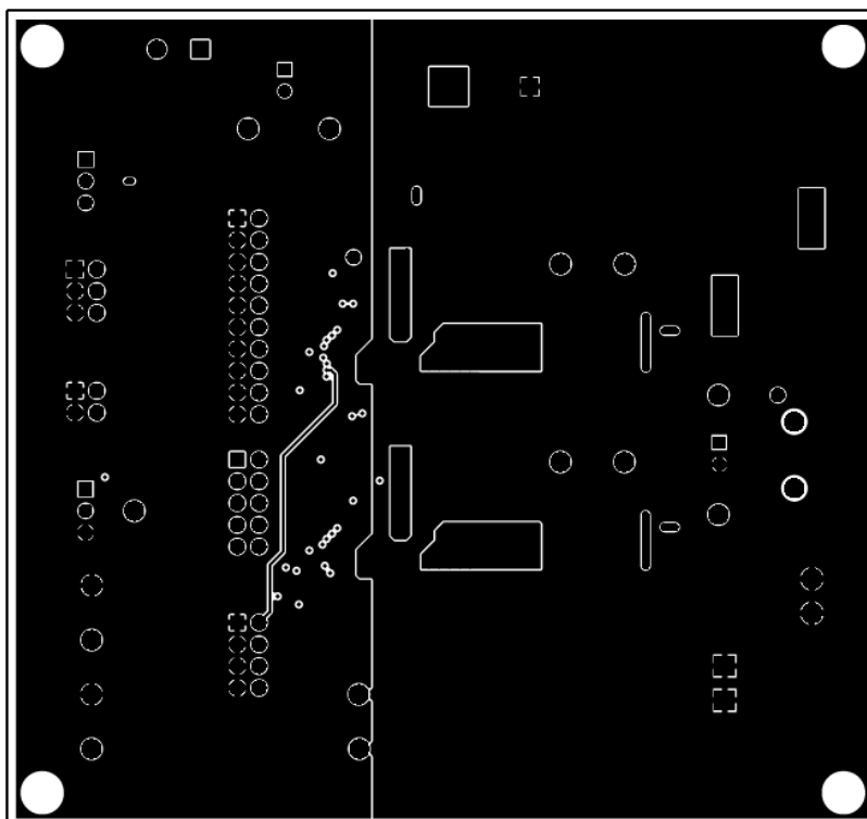
Figure 4-8. Signal Layer 6
