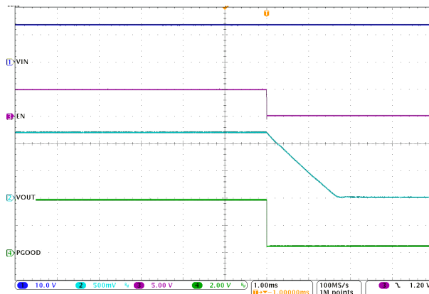
Figure 3-2. ENABLE Shutdown Waveform
