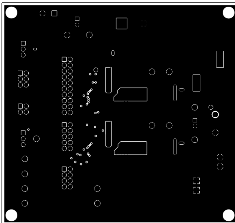
Figure 4-3. Signal Layer 1
