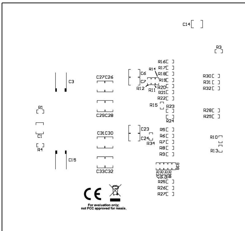
Figure 4-10. Bottom Layer Silk Screen (Bottom View)
