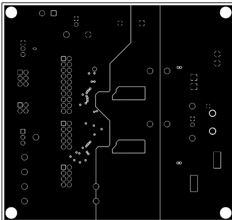
Figure 4-4. Signal Layer 2
