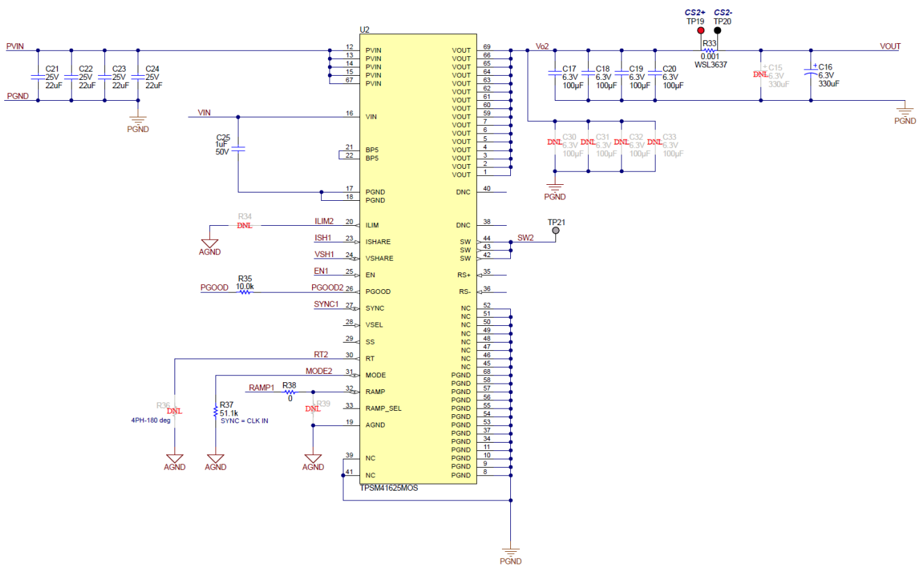
Figure 5-2. Secondary Schematic
