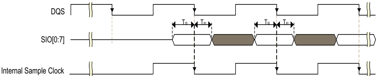
Fig 23. SDR mode (input timing, mode 3)
