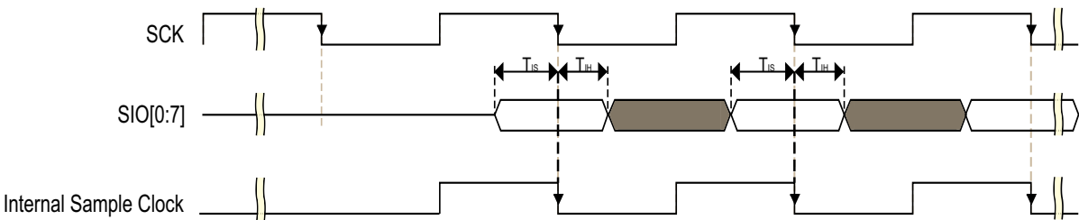
Fig 22. SDR mode (input timing, mode 0 and 1)
