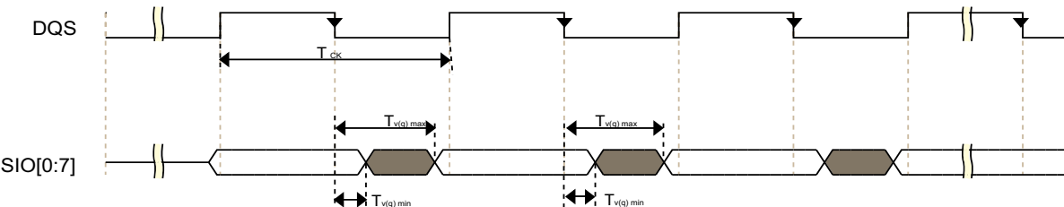
Fig 25. SDR mode (output timing, mode 3)
