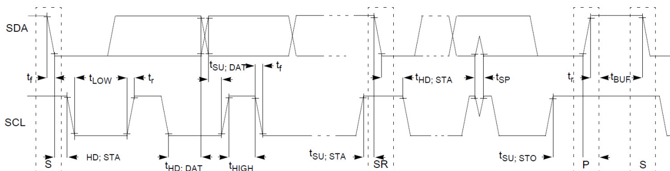
Fig 14. Timing definition for devices on the I 2 C bus
