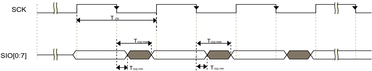
Fig 24. SDR mode (output timing, mode 0 and 1)
