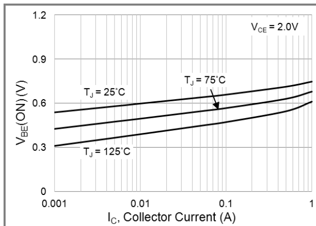
Fig.2 Typical Base-Emitter Turn-on Voltage
