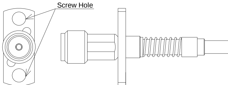
Figure.2 Screw hole size
