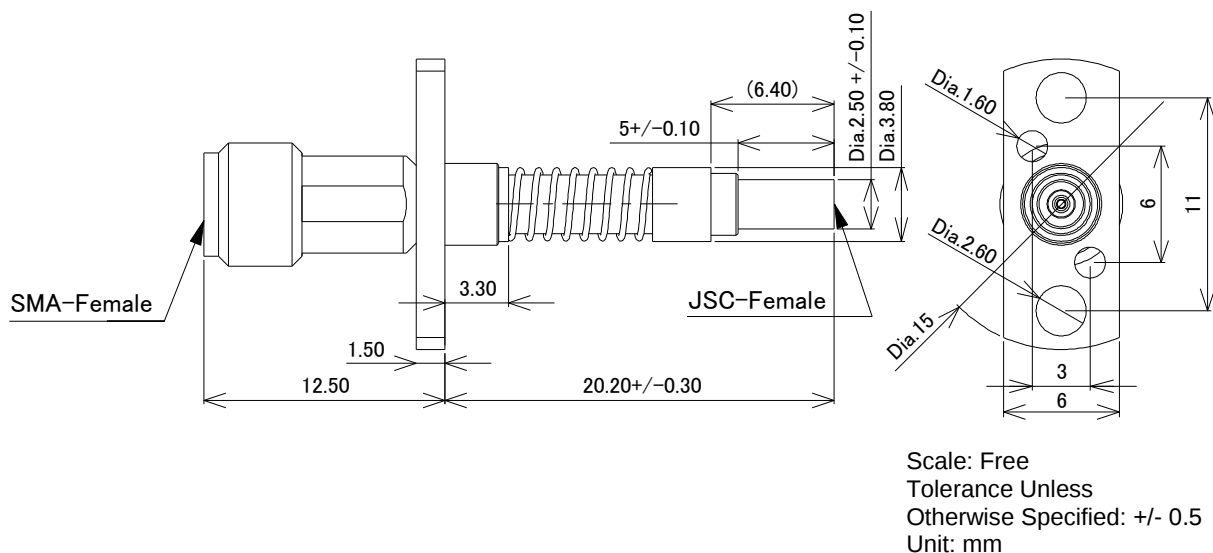
Figure.1 Construction
