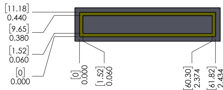
TRACE PATTERN SCALE 1:1
