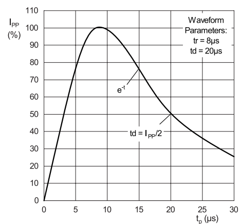
Fig. 3. Pulse waveform
