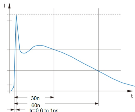
IEC61000-4-2 Waveform
