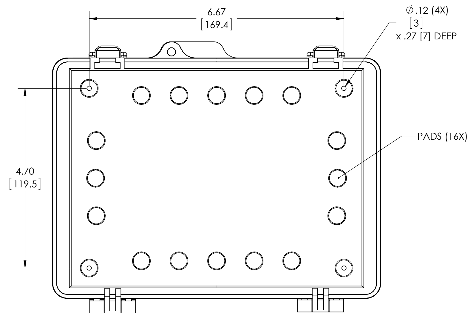
BOTTOM VIEW
