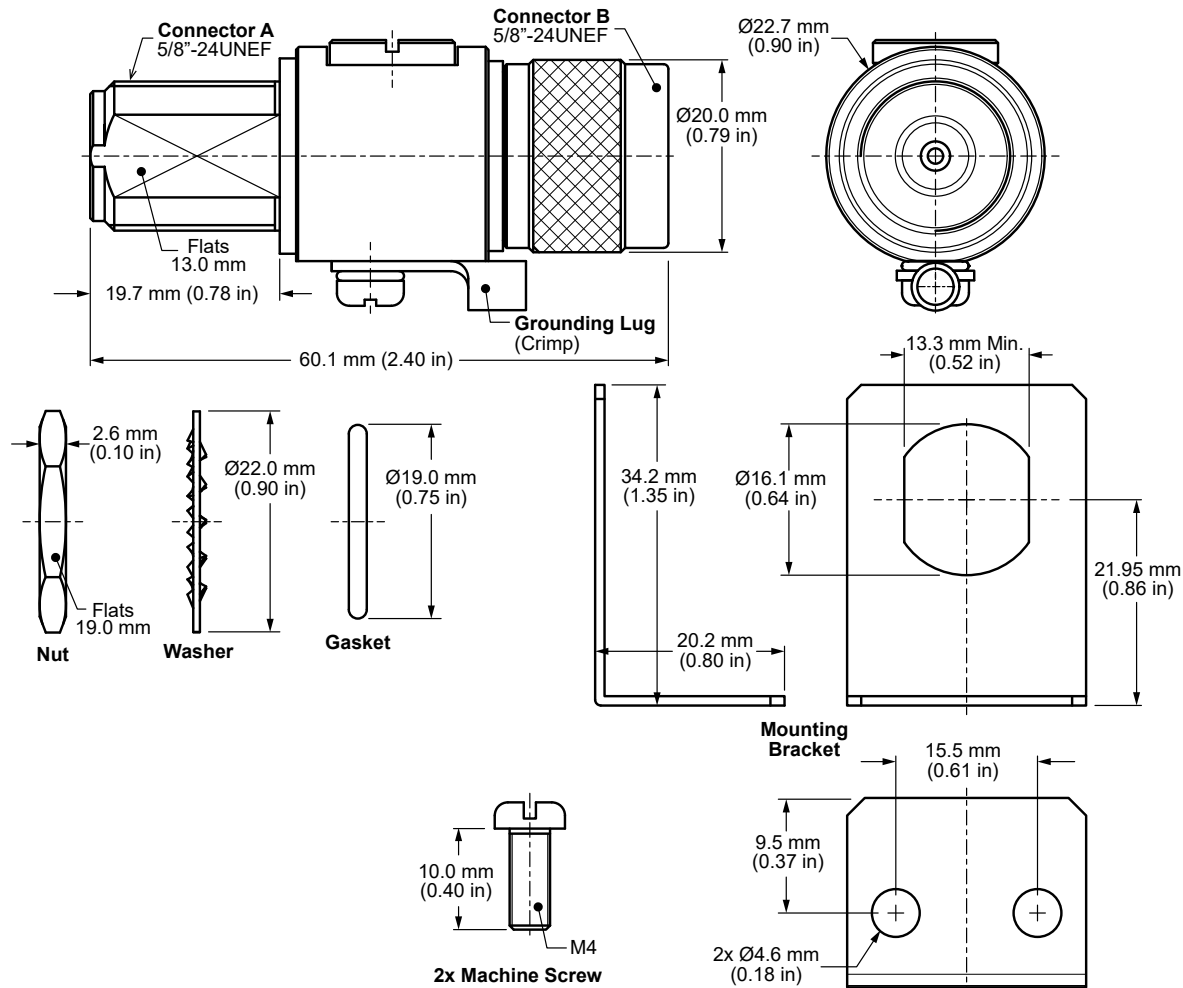
Figure 1. Product Dimensions for the ARR-NF-NM-B Lightning Arrester
