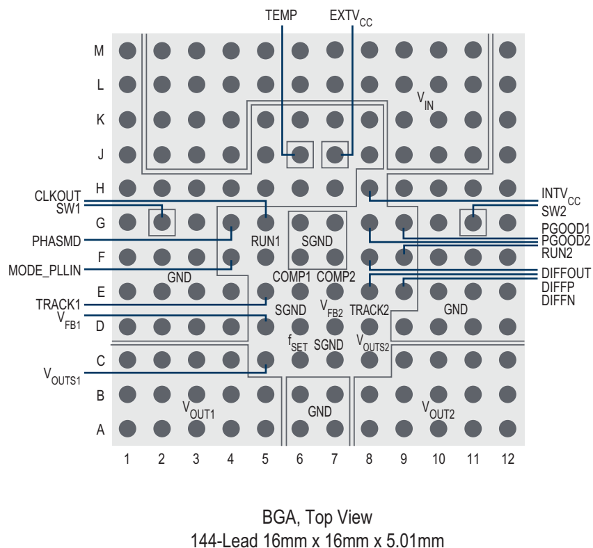
Figure 3: Pin Configuration
