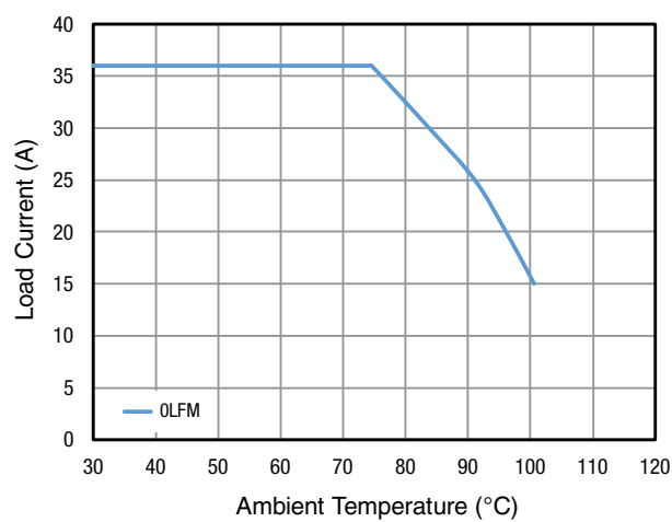
Figure 38: 12V to 1V Current Derating
