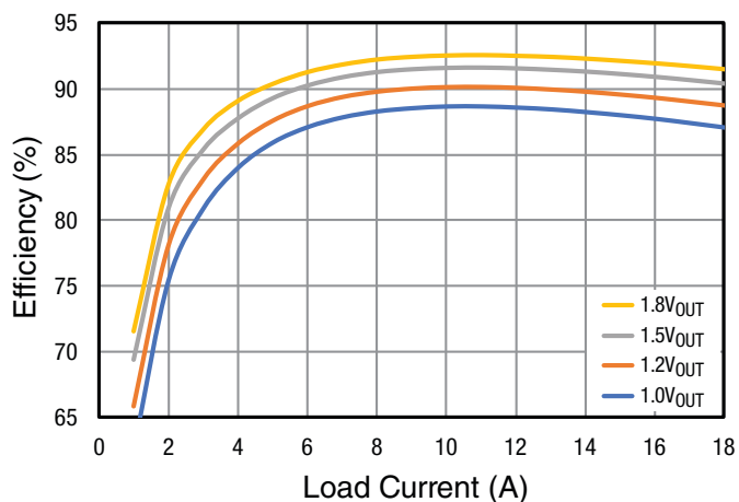
Figure 5: Efficiency: Single Phase, V_{IN} = 12V , 450kHz
