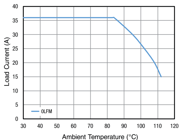
Figure 40: 5V to 1V Current Derating
