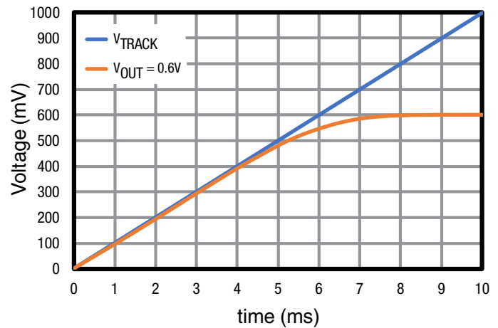
Figure 23: V_{OUT} and V_{\text{TRACK}} versus Time
