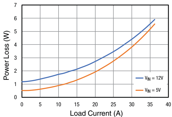
Figure 36: 1.5V Output Power Loss
