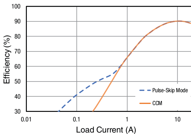
Figure 7: Efficiency: Pulse-Skipping Mode, V_{IN} = 12V , V_{OUT} = 1.2V , 450kHz
