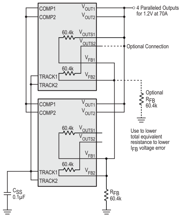
Figure 19: 4-Phase Parallel Configuration
