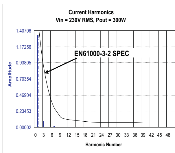
Figure 7. Current Harmonics
