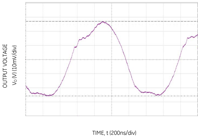
Figure 33. Typical output ripple and noise ( C_o=1 \times 47 \mu\text{F} ceramic, V_{IN} = 12\text{V} , I_o = I_{o,max} ).
