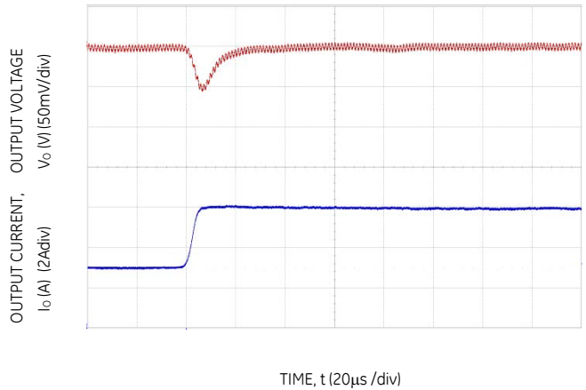
Figure 22. Transient Response to Dynamic Load Change from 50% to 100% at 12V in , C out = 4x47μF, C Tune =2700pF & R Tune =300Ω
