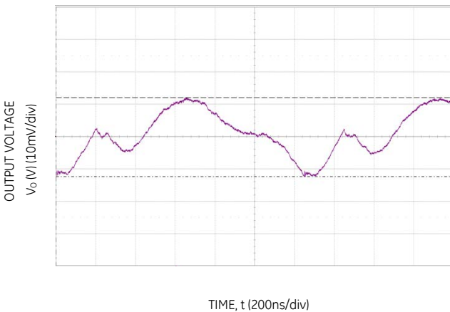
Figure 15. Typical output ripple and noise ( C_o=1 \times 47 \mu F ceramic, V_{IN} = 12V , I_o = I_{o,max} ).
