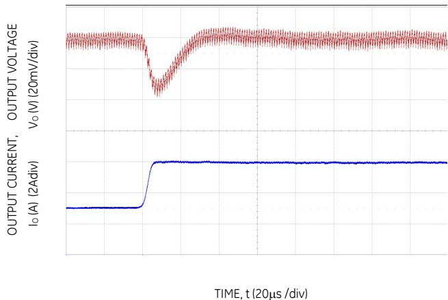
Figure 16. Transient Response to Dynamic Load Change from 50% to 100% at 12Vin, C_{out} = 2 \times 47 \mu F + 1 \times 330 \mu F , C_{Tune}=2700pF & R_{Tune}=300\Omega
