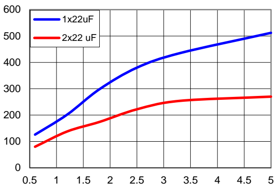
Figure 37. Input ripple voltage for various output voltages with 1x22 μF or 2x22 μF ceramic capacitors at the input (6A load). Input voltage is 12V.
