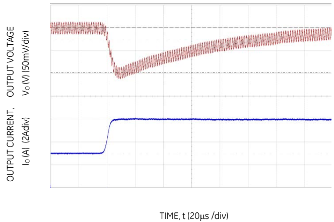
Figure 34. Transient Response to Dynamic Load Change from 50% to 100% at 12Vin, C_{out} = 3 \times 47 \mu\text{F} , C_{Tune} = 1500\text{pF} & R_{Tune} = 300 \Omega
