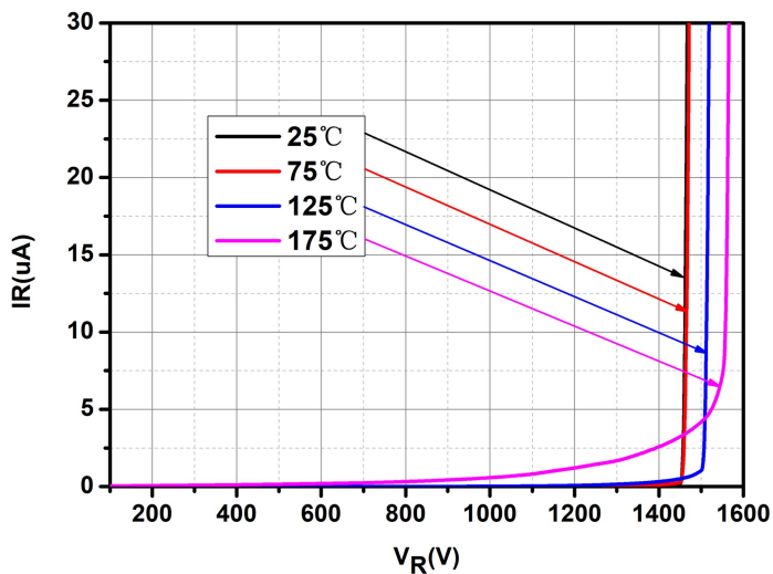
Fig.2-Typical Reverse Characteristics
