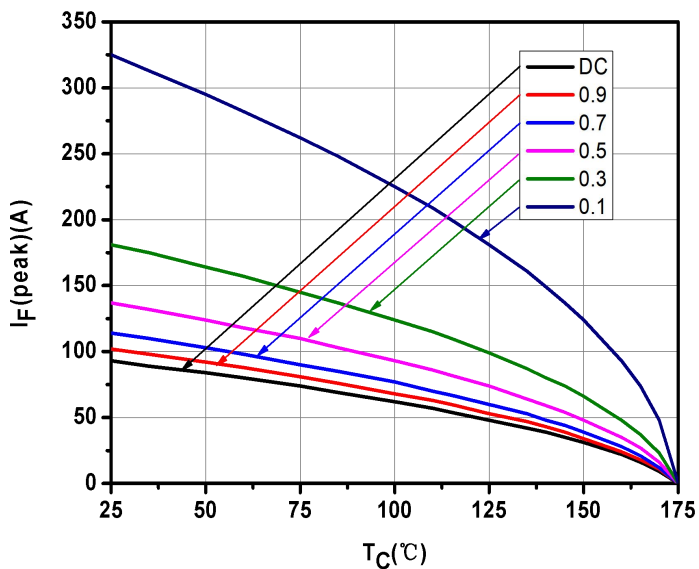
Fig.4-Current Derating
