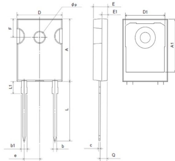
TO-247-2L, (TO-247GE-2L)
