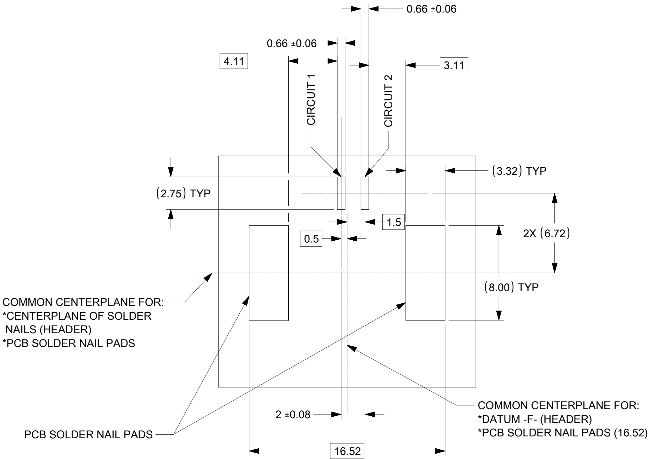
PCB LAYOUT
