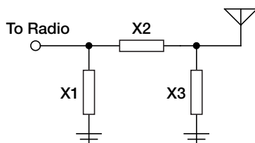
Figure 9. Matching Network Recommendation
