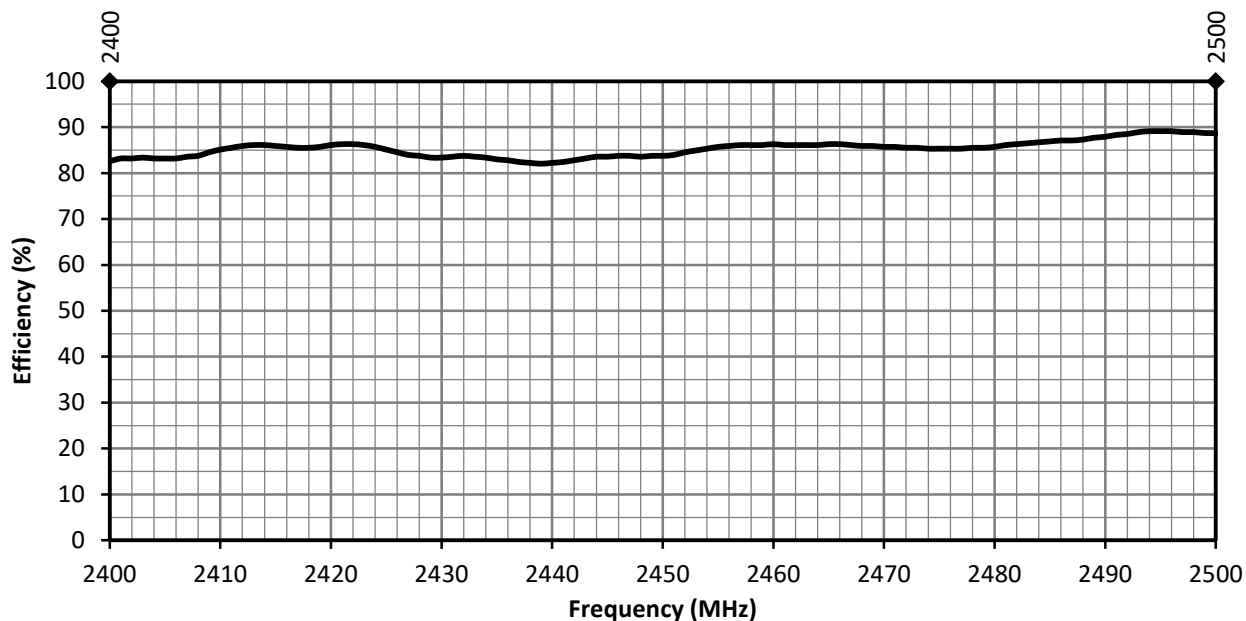
Figure 7. ANT-2.4-MSA-TH1 Radiation Efficiency
