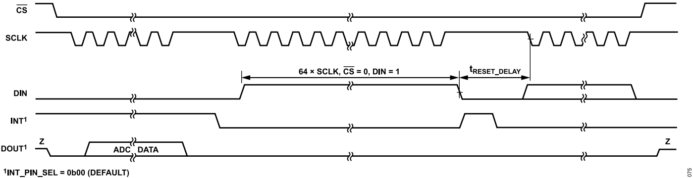
Figure 75. Software Reset Timing Diagram
