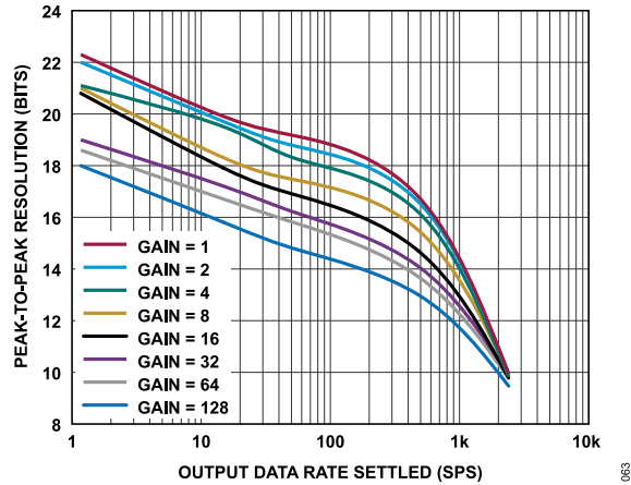
Figure 63. Peak-to-Peak Resolution vs. Output Data Rate (Settled) for Various Gains ( \text{Sinc}^3 Filter)
