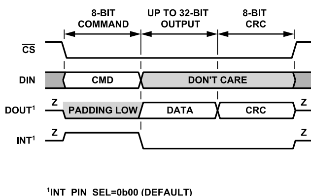
Figure 100. SPI Read Transaction with CRC
