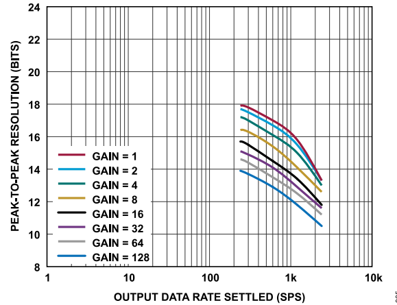
Figure 65. Peak-to-Peak Resolution vs. Output Data Rate (Settled) for Various Gains ( \text{Sinc}^4 Filter)
