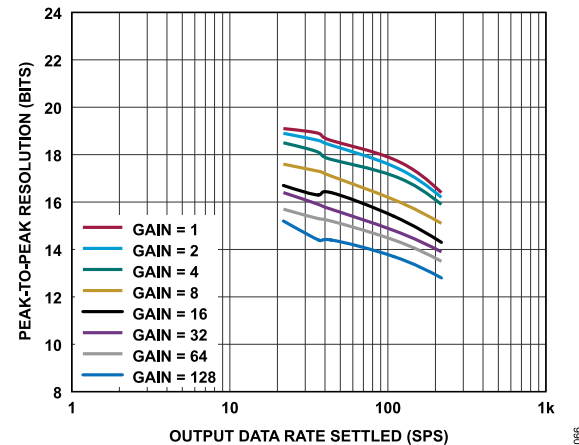
Figure 66. Peak-to-Peak Resolution vs. Output Data Rate (Settled) for Various Gains ( \text{Sinc}^4 + \text{Sinc}^1 Filter)
