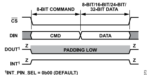
Figure 73. Writing to a Register (8-Bit Command with Register Address Followed by Data)
