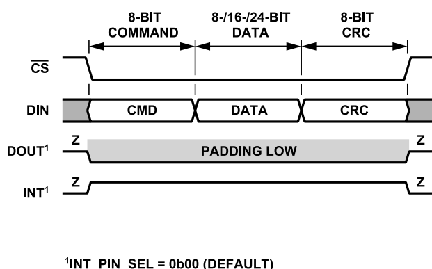
Figure 99. SPI Write Transaction with CRC
