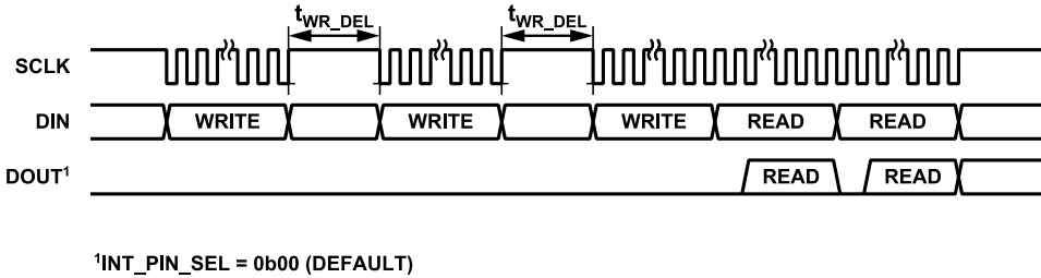
Figure 4. Delay Between Consecutive Serial Operations, 3-Wire Mode (CSB_EN Bit Set to 0), CS Pin Tied Low
