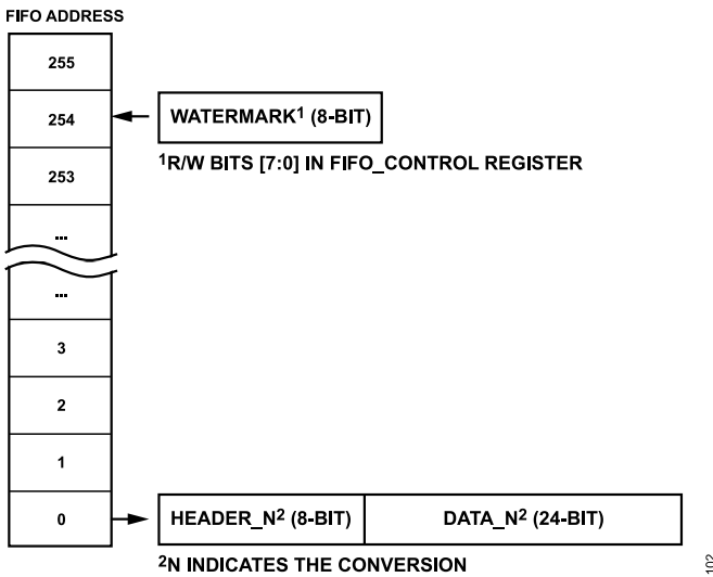
Figure 102. FIFO Structure
