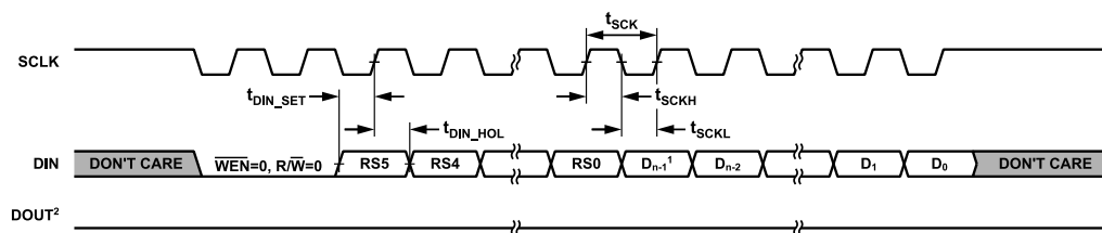
Figure 2. Write Cycle Timing Diagram, 3-Wire Mode (CSB_EN Bit Set to 0), \overline{\text{CS}} Pin Tied Low
