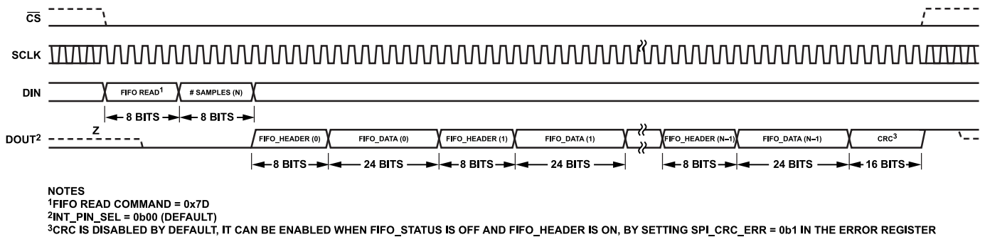
Figure 106. FIFO Readback (FIFO_STATUS Append Off and FIFO_HEADER Append On, CRC On)
