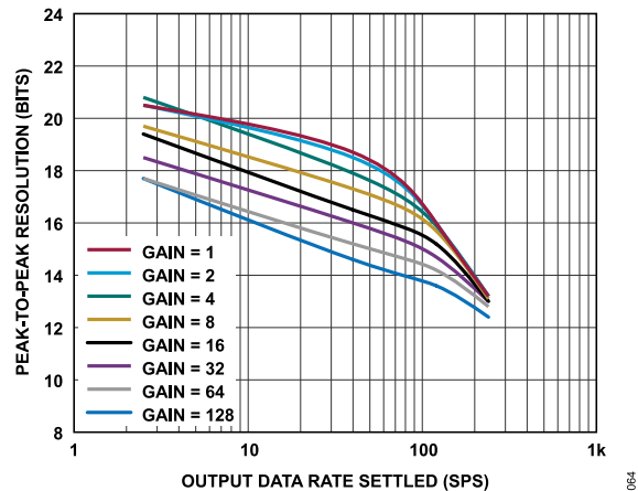
Figure 64. Peak-to-Peak Resolution vs. Output Data Rate (Settled) for Various Gains ( \text{Sinc}^3 + \text{Sinc}^1 Filter)
