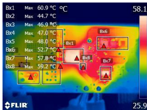
Figure 36 – Bottom Components, Ambient = 27 °C.
