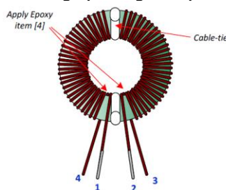
Figure 12 – Inductor Illustration
