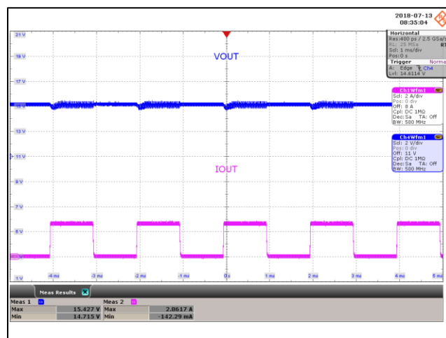
Figure 62 – Transient Response. 265 VAC, 15.0 V, 0 - 2.66 A Load Step. V_{\text{MIN}} : 14.71 V, V_{\text{MAX}} : 15.42 V. Upper: V_{\text{OUT}} , 2 V / div., 1 ms / div. Lower: I_{\text{LOAD}} , 2 A / div.
