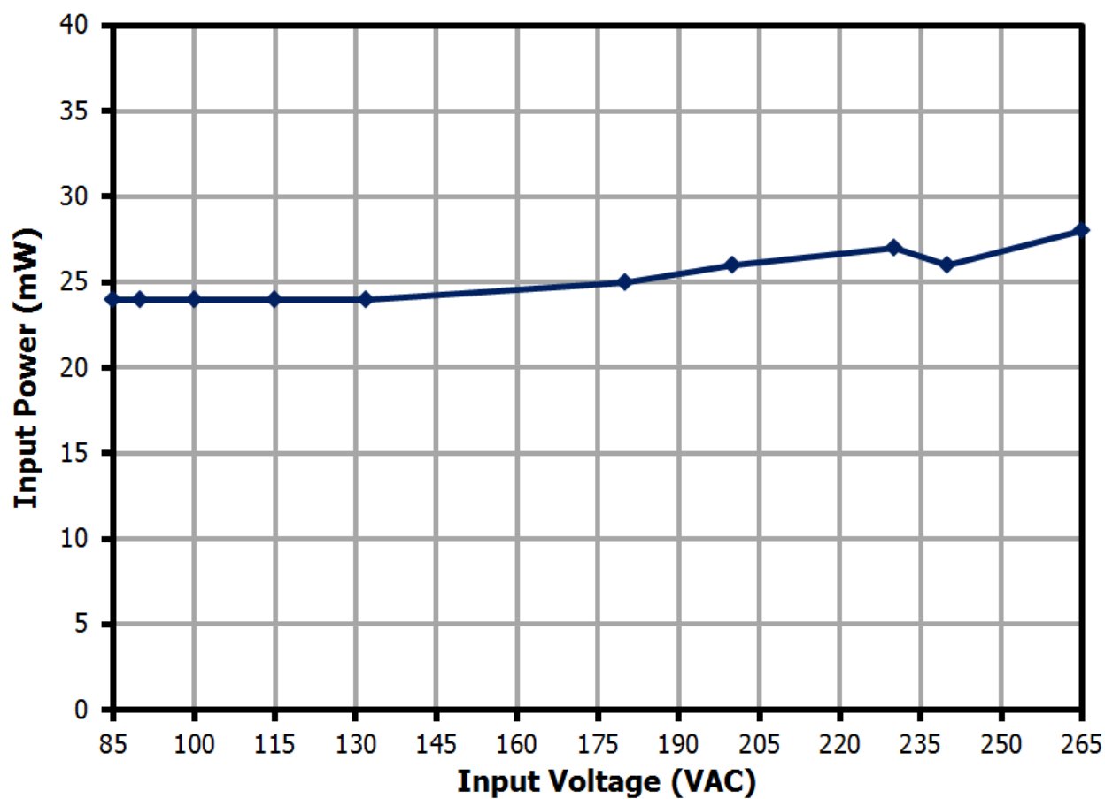
Figure 29 – No-Load Input Power vs. Input Line Voltage, Room Temperature.
