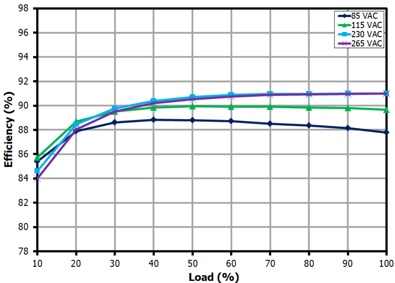
Figure 16 – Efficiency vs. Load, Room Ambient.
