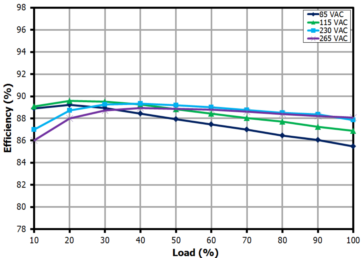
Figure 14 – Efficiency vs. Load, Room Ambient.
