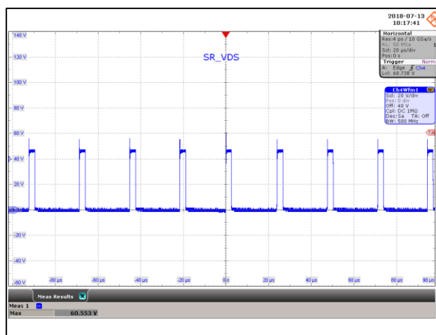
Figure 80 – SR FET Voltage Waveforms. 265 VAC, 5.0 V, 5 A Load (60.53 V MAX ). SR_V DRAIN , 20 V / div., 20 μs / div.
