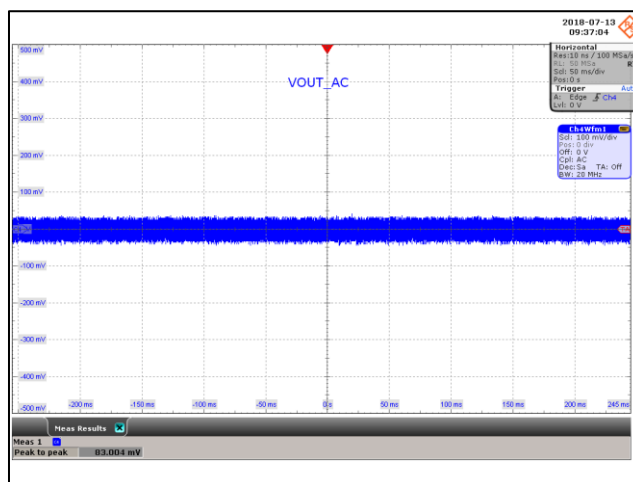
Figure 98 – Output Ripple.(PK-PK – 83 mV). 265 VAC Input 15.0 V, 2.66 A Load. V_{OUT} , 100 mV / div., 50 ms / div.
