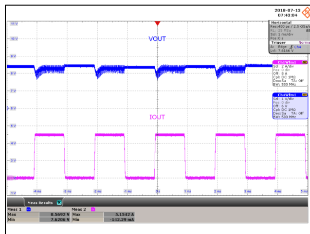
Figure 60 – Transient Response. 265 VAC, 8.0 V, 0 - 5 A Load Step. V_{\text{MIN}} : 7.62 V, V_{\text{MAX}} : 8.56 V. Upper: V_{\text{OUT}} , 1 V / div., 1 ms / div. Lower: I_{\text{LOAD}} , 2 A / div.
