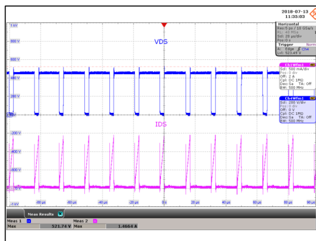
Figure 70 – Drain Voltage and Current Waveforms. 265 VAC, 8.0 V, 5 A Load (521 V MAX ). Upper: V DRAIN , 200 V / div., 20 μs / div. Lower: I DRAIN , 500 mA / div.
