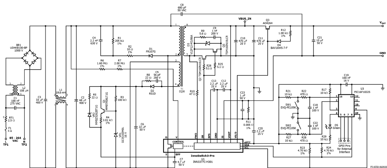
Figure 3 – Schematic.
