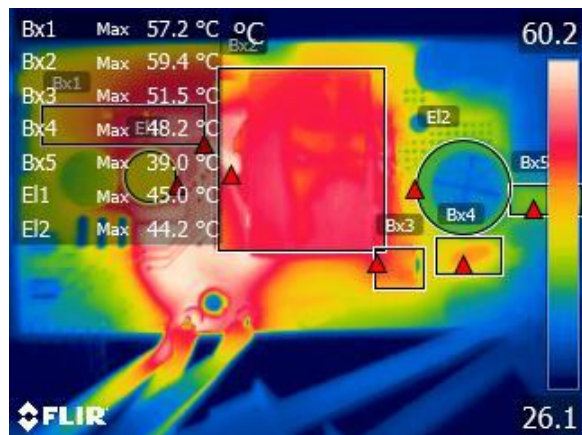
Figure 41 – Top Components, Ambient = 27 °C.
