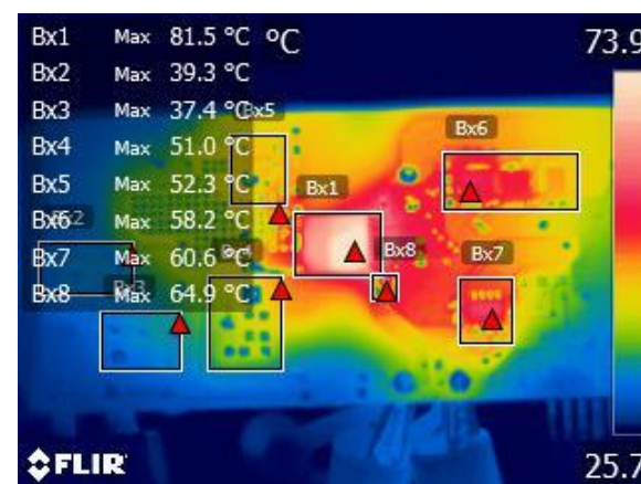
Figure 38 – Bottom Components, Ambient = 27 °C.
