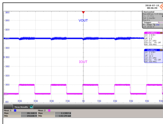
Figure 64 – Transient Response.
