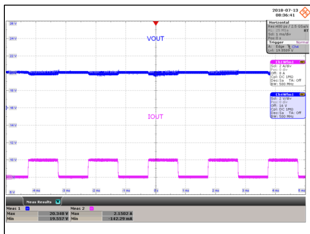
Figure 63 – Transient Response.
