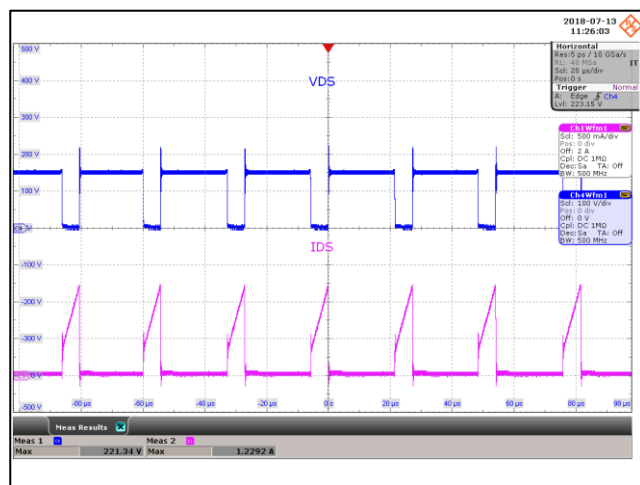
Figure 65 – Drain Voltage and Current Waveforms. 85 VAC, 3.0 V, 5 A Load (221 V MAX ). Upper: V DRAIN , 100 V / div., 20 µs / div. Lower: I DRAIN , 500 mA / div.
