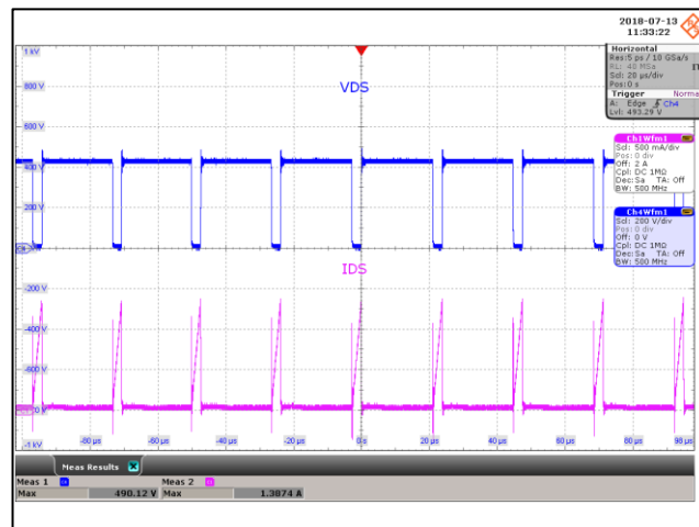
Figure 68 – Drain Voltage and Current Waveforms. 265 VAC, 5.0 V, 5 A Load (490 V MAX ). Upper: V DRAIN , 200 V / div., 20 µs / div. Lower: I DRAIN , 500 mA / div.
