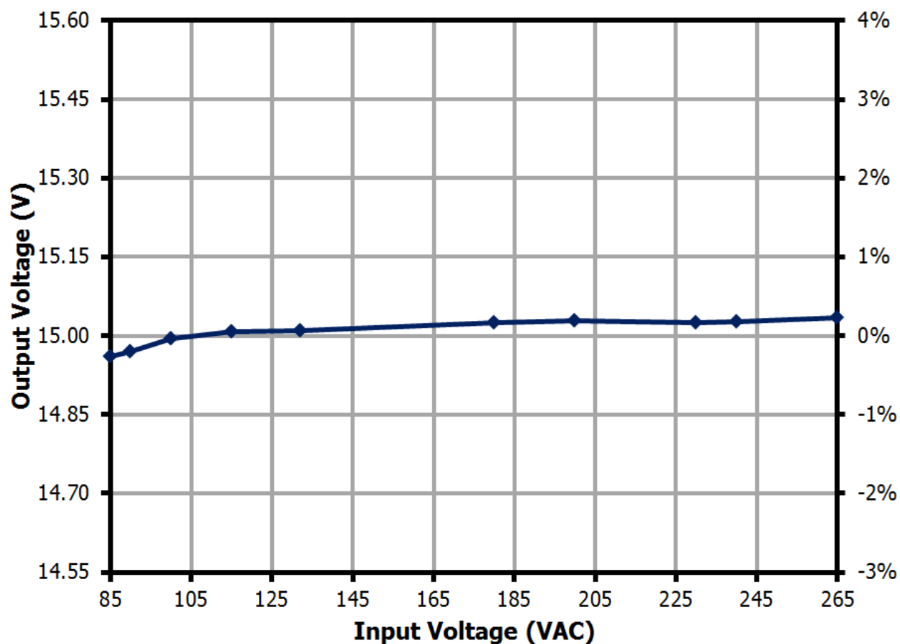
Figure 22 – 15 V Output Regulation vs. Input Line Voltage.
