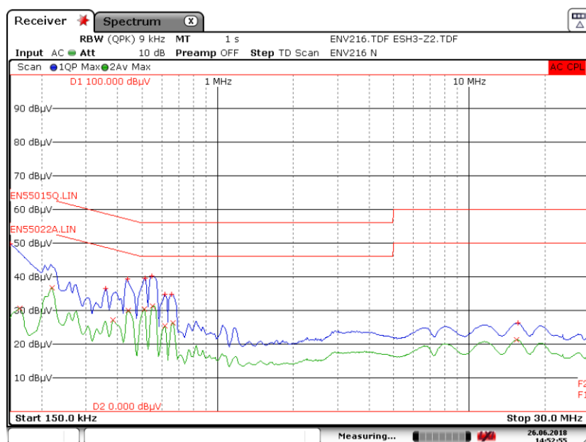
Figure 106 – Floating Ground EMI, 20 V / 2 A Load 115 VAC, 60 Hz, and EN55022 B Limits (Neutral).
