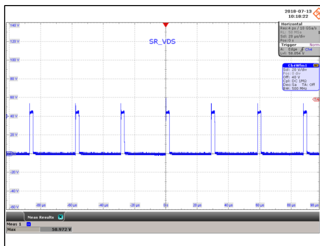
Figure 78 – SR FET Voltage Waveforms. 265 VAC, 3.0 V, 5 A Load (58.97 V MAX ). SR_V DRAIN , 20 V / div., 20 μs / div.
