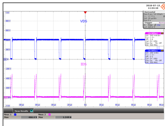
Figure 66 – Drain Voltage and Current Waveforms. 265 VAC, 3.0 V, 5 A Load (466 V MAX ). Upper: V DRAIN , 200 V / div., 20 µs / div. Lower: I DRAIN , 500 mA / div.
