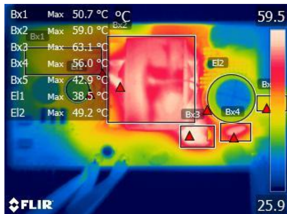
Figure 49 – Top Components, Ambient = 27 °C.
