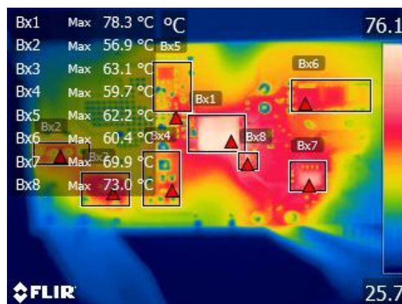
Figure 40 – Bottom Components, Ambient = 27 °C.
