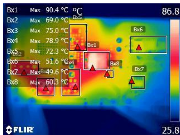
Figure 48 – Bottom Components, Ambient = 27 °C.
