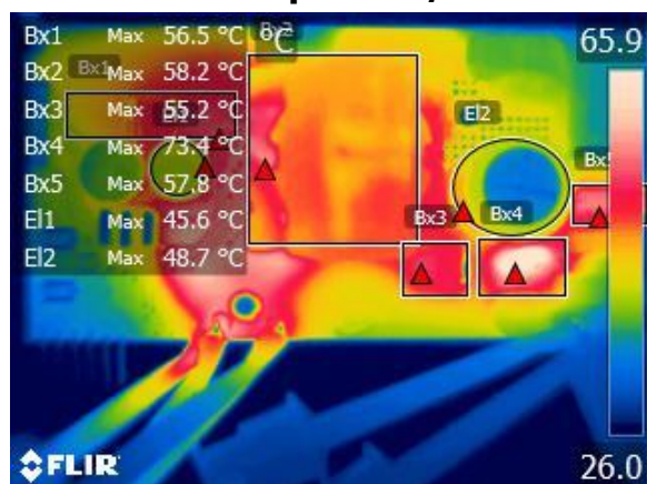
Figure 39 – Top Components, Ambient = 27 °C.
