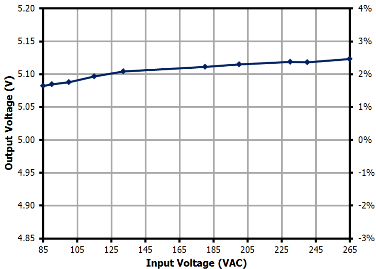
Figure 20 – 5 V Output Regulation vs. Input Line Voltage.
