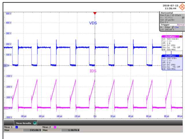
Figure 67 – Drain Voltage and Current Waveforms. 85 VAC, 5.0 V, 5 A Load (245 V MAX ). Upper: V DRAIN , 100 V / div., 20 µs / div. Lower: I DRAIN , 500 mA / div.
