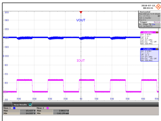
Figure 61 – Transient Response. 85 VAC, 15.0 V, 0 - 2.66 A Load Step. V_{\text{MIN}} : 14.55 V, V_{\text{MAX}} : 15.42 V. Upper: V_{\text{OUT}} , 2 V / div., 1 ms / div. Lower: I_{\text{LOAD}} , 2 A / div.
