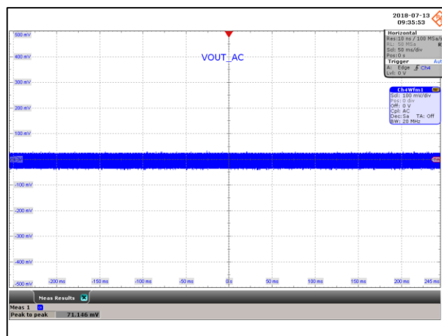
Figure 96 – Output Ripple.(PK-PK – 71 mV). 265 VAC Input 8.0 V, 5 A Load. V_{OUT} , 100 mV / div., 50 ms / div.
