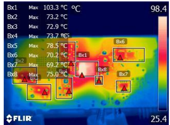
Figure 44 – Bottom Components, Ambient = 27 °C.
