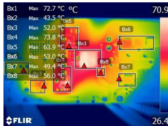
Figure 50 – Bottom Components, Ambient = 27 °C.
