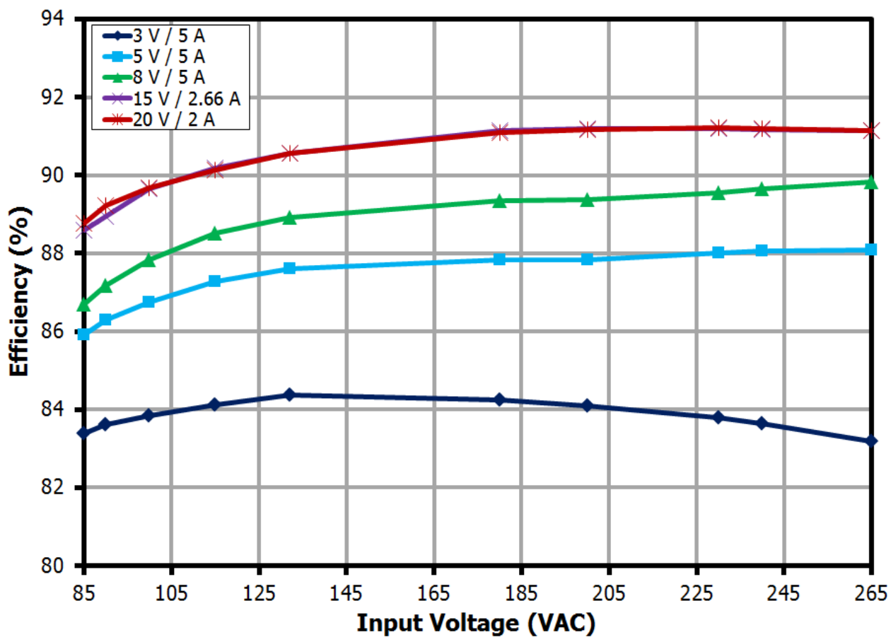
Figure 18 – Efficiency vs. Line, Room Ambient.
