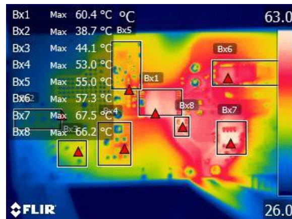
Figure 42 – Bottom Components, Ambient = 27 °C.
