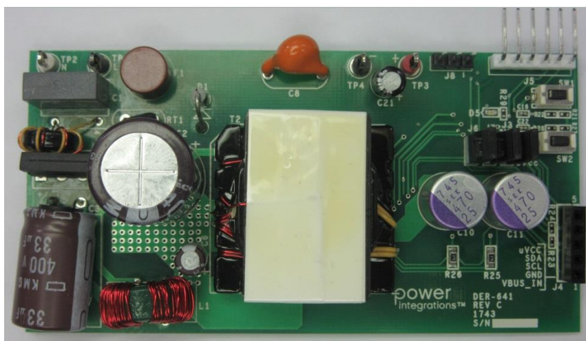
Figure 1 – Populated Circuit Board Photograph, Top. (DER-641 is equivalent to RD-641.)
