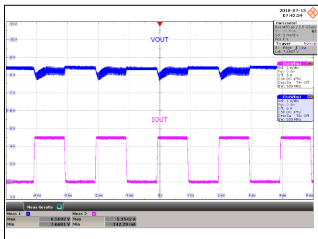
Figure 59 – Transient Response. 85 VAC, 8.0 V, 0 - 5 A Load Step. V_{\text{MIN}} : 7.66 V, V_{\text{MAX}} : 8.56 V. Upper: V_{\text{OUT}} , 1 V / div., 1 ms / div. Lower: I_{\text{LOAD}} , 2 A / div.
