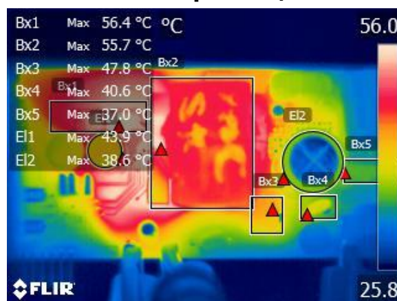
Figure 37 – Top Components, Ambient = 27 °C.
