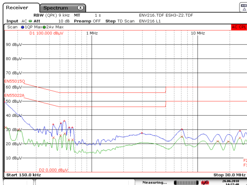
Figure 105 – Floating Ground EMI, 20 V / 2 A Load 115 VAC, 60 Hz, and EN55022 B Limits (Line).
