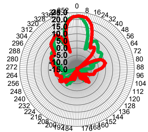
Antenna Pattern
