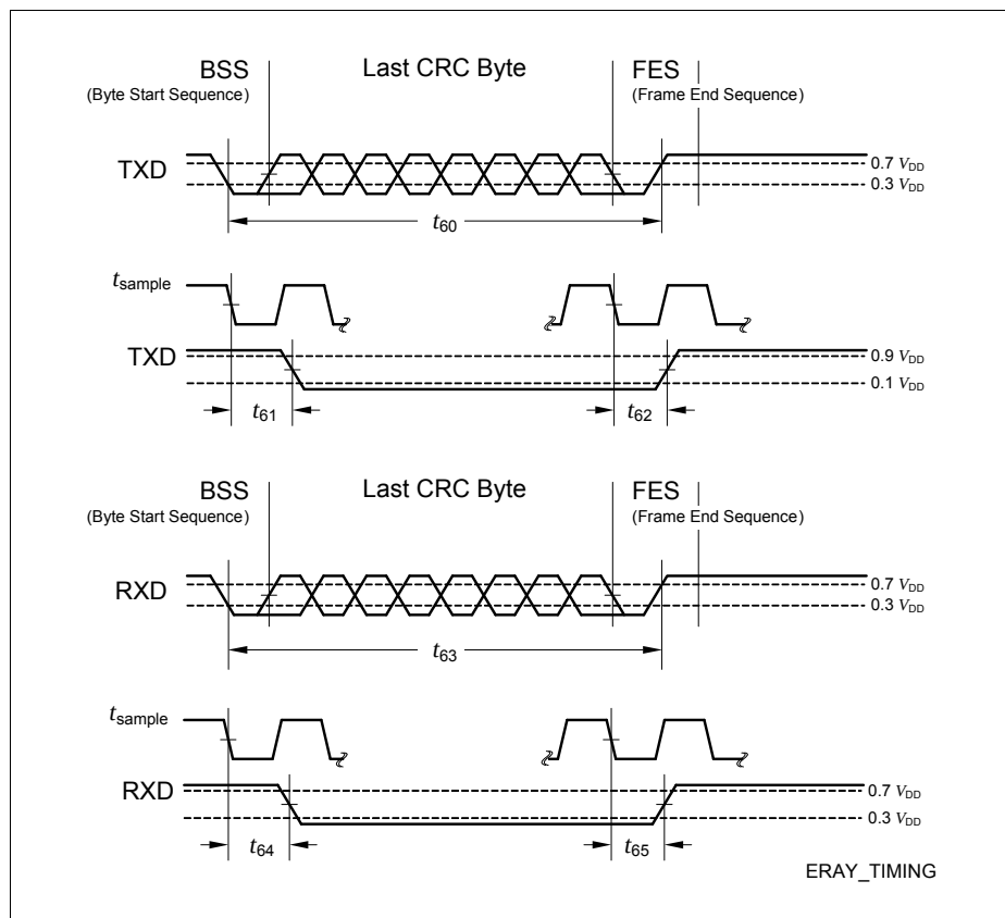
Figure 22 ERAY Timing
